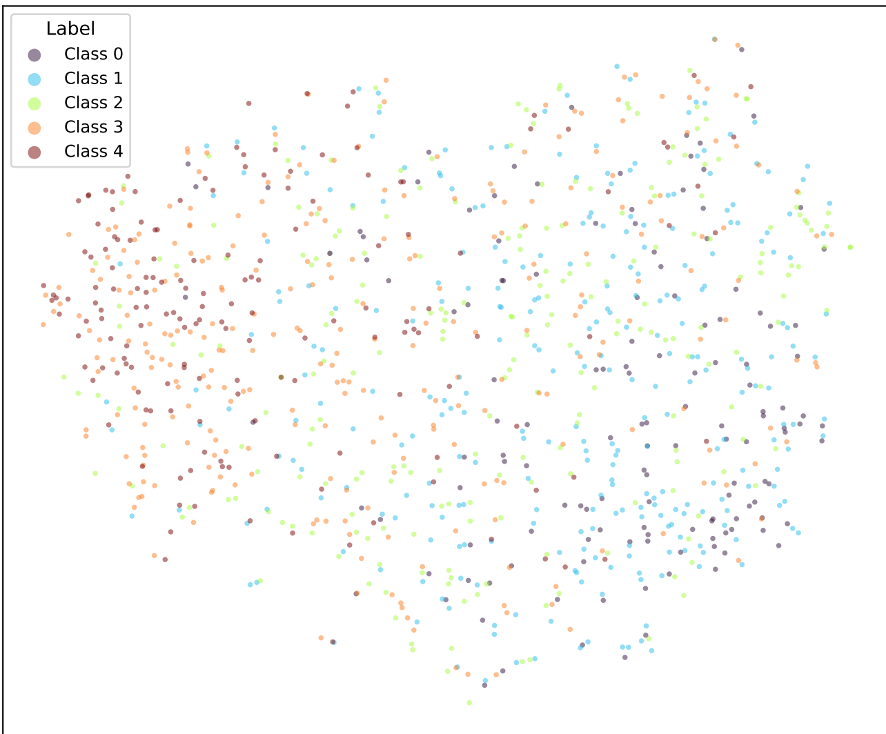
t-SNE | bert-tiny-sst5-k10-adaptive-cosine (epoch 5.0)
