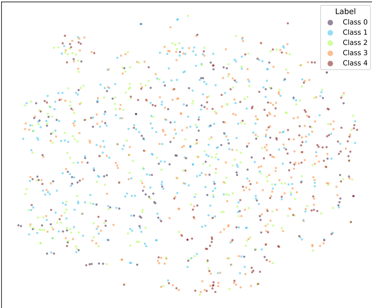
t-SNE | bert-tiny-sst5-k3-fixed-cosine
