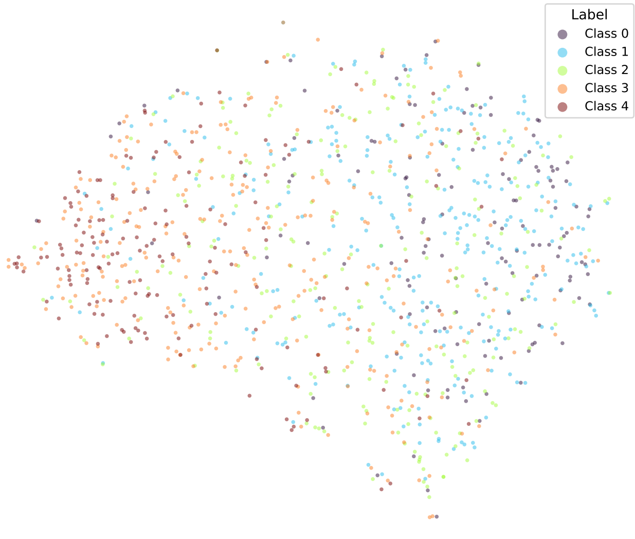
t-SNE | bert-tiny-sst5-k5-adaptive-cosine
