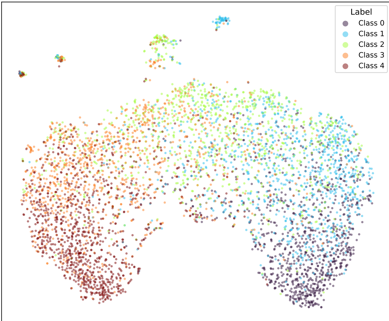
t-SNE | bert-tiny-yelp-k1-fixed-cosine
