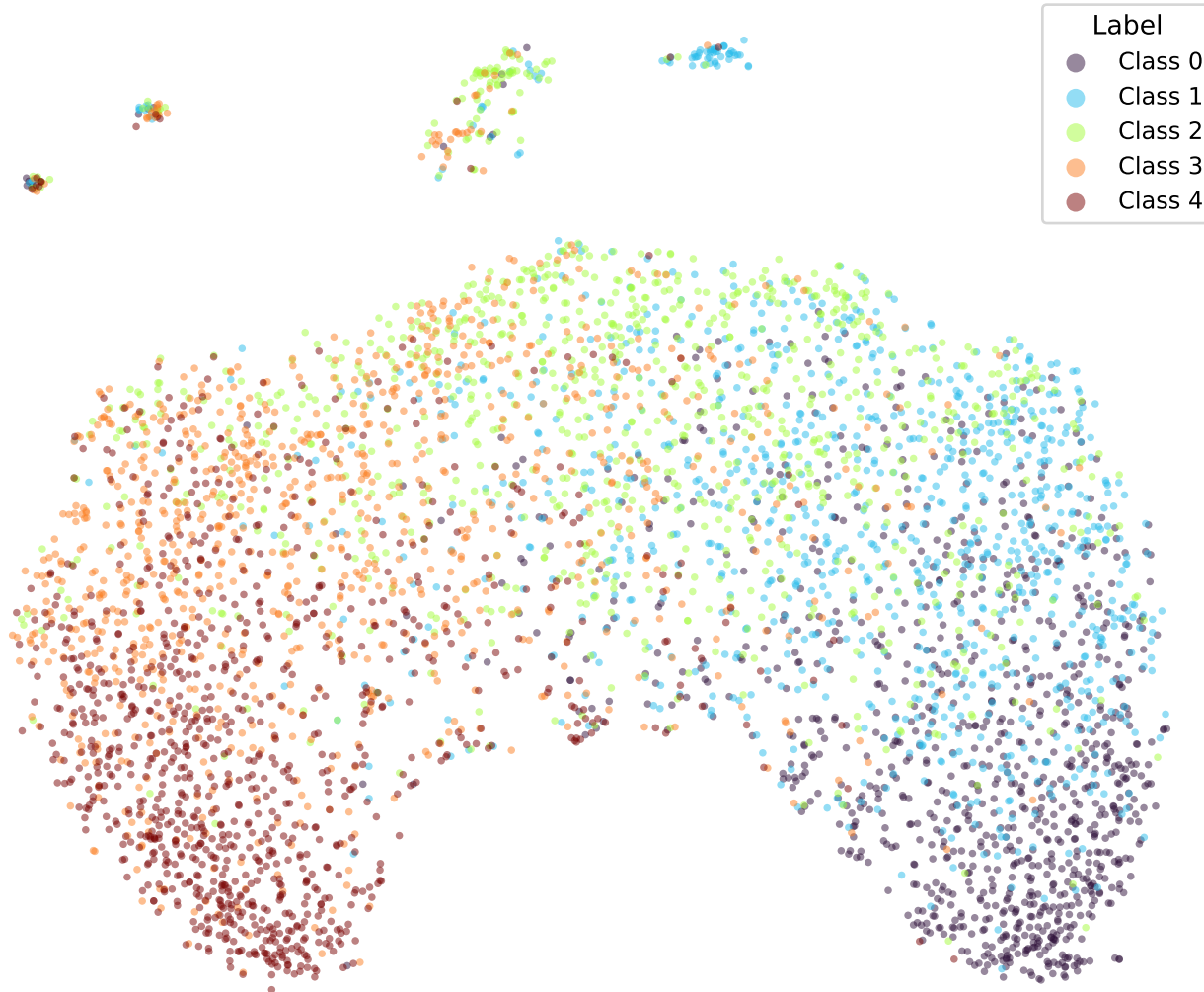
t-SNE | bert-tiny-yelp-k1-fixed-cosine (epoch 5.0)
