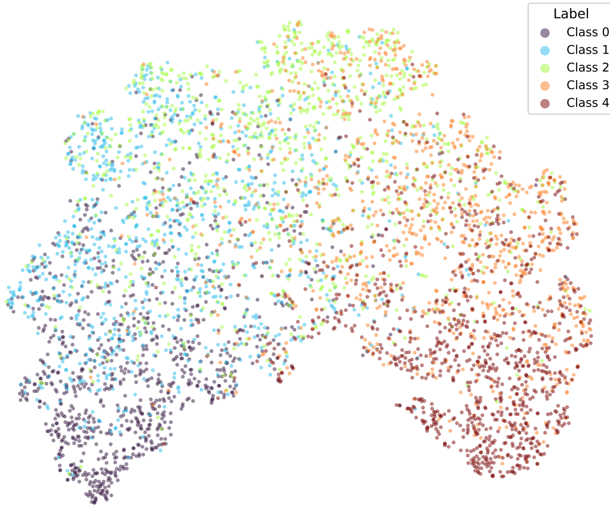
t-SNE | bert-tiny-yelp-k1-fixed-euclidean (epoch 3.0)
