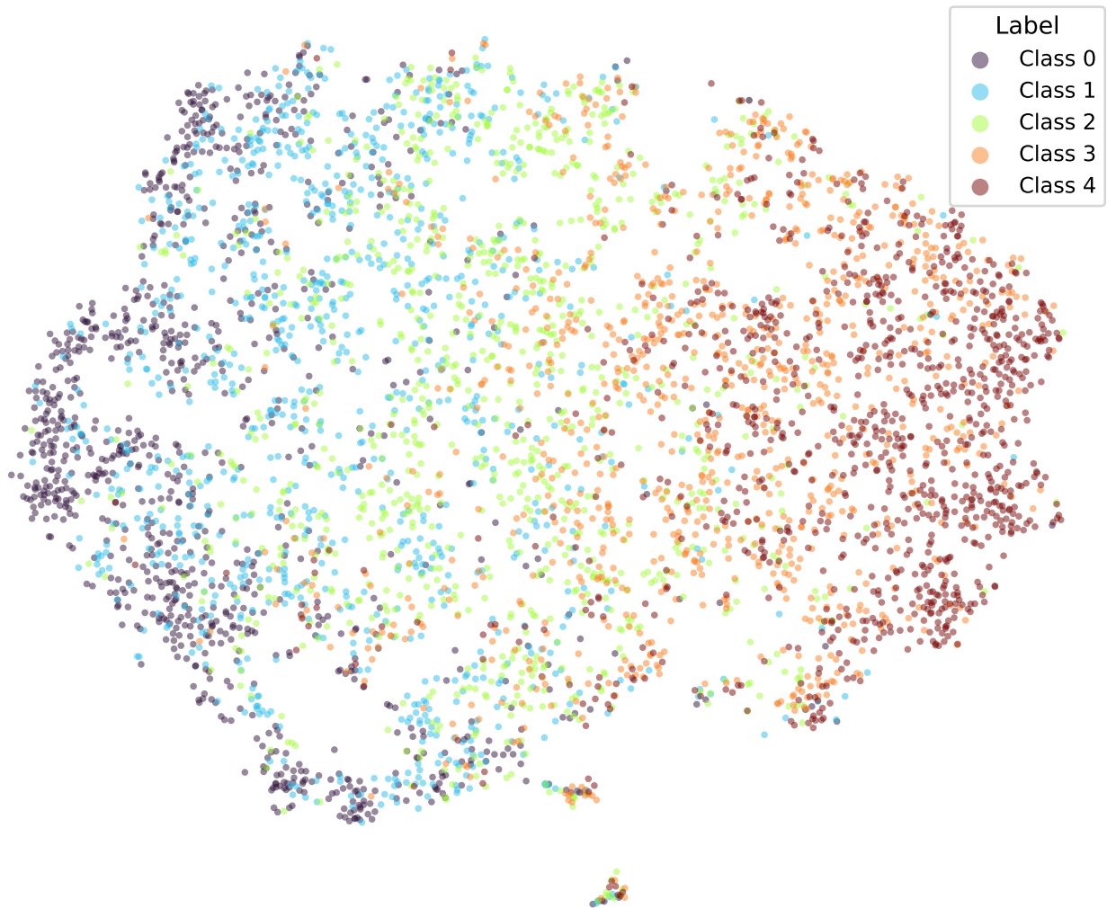
t-SNE | bert-tiny-yelp-k3-adaptive-cosine (epoch 3.0)
