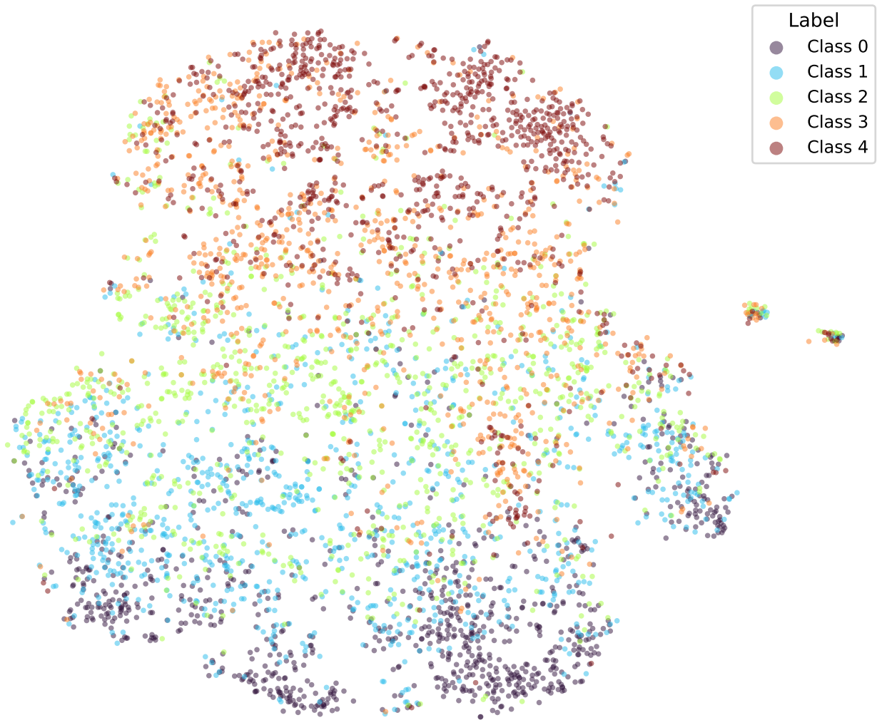
t-SNE | bert-tiny-yelp-k3-fixed-cosine (epoch 7.0)
