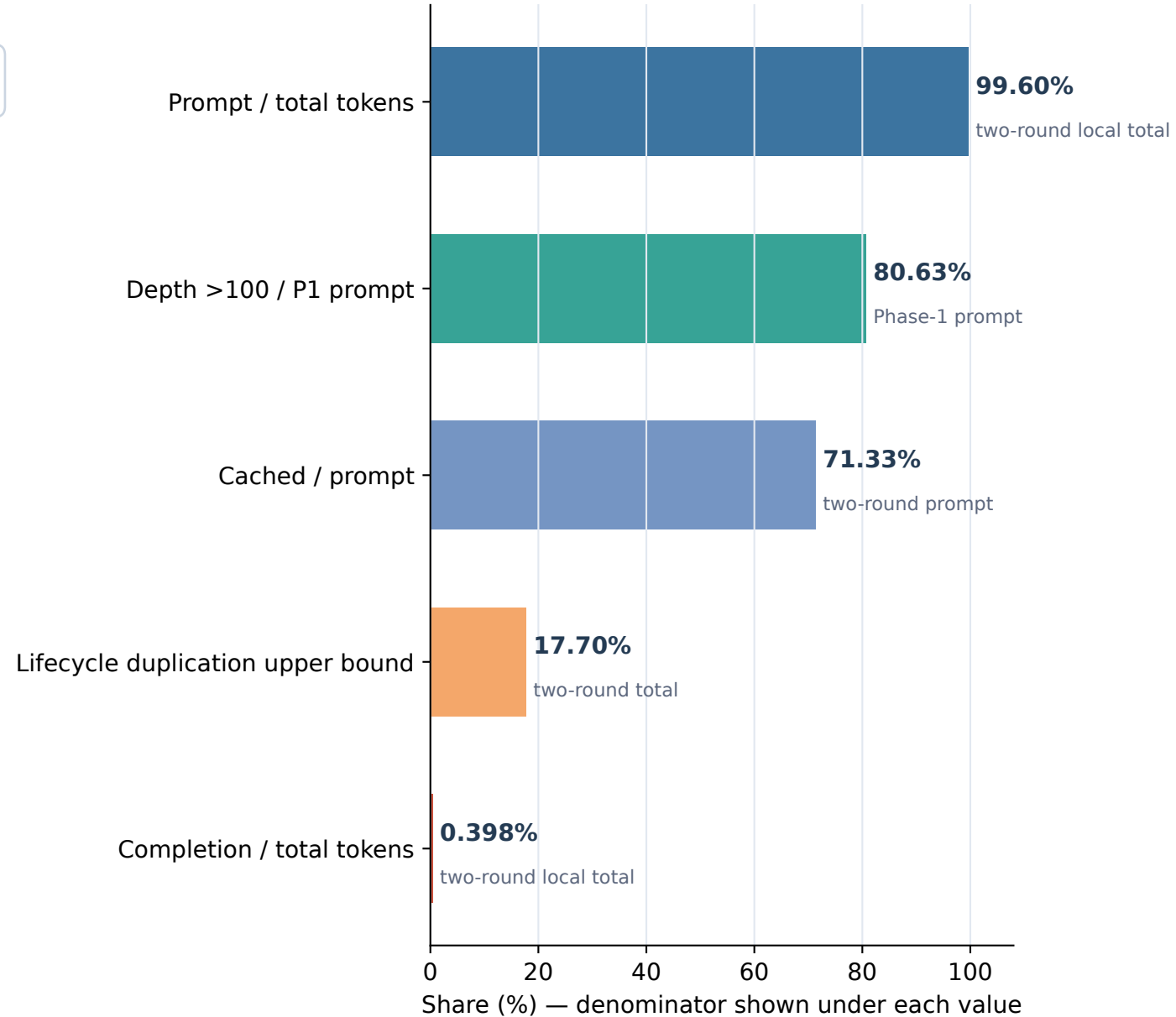
B. Local recorded usage is prompt-heavy, with avoidable overlap
