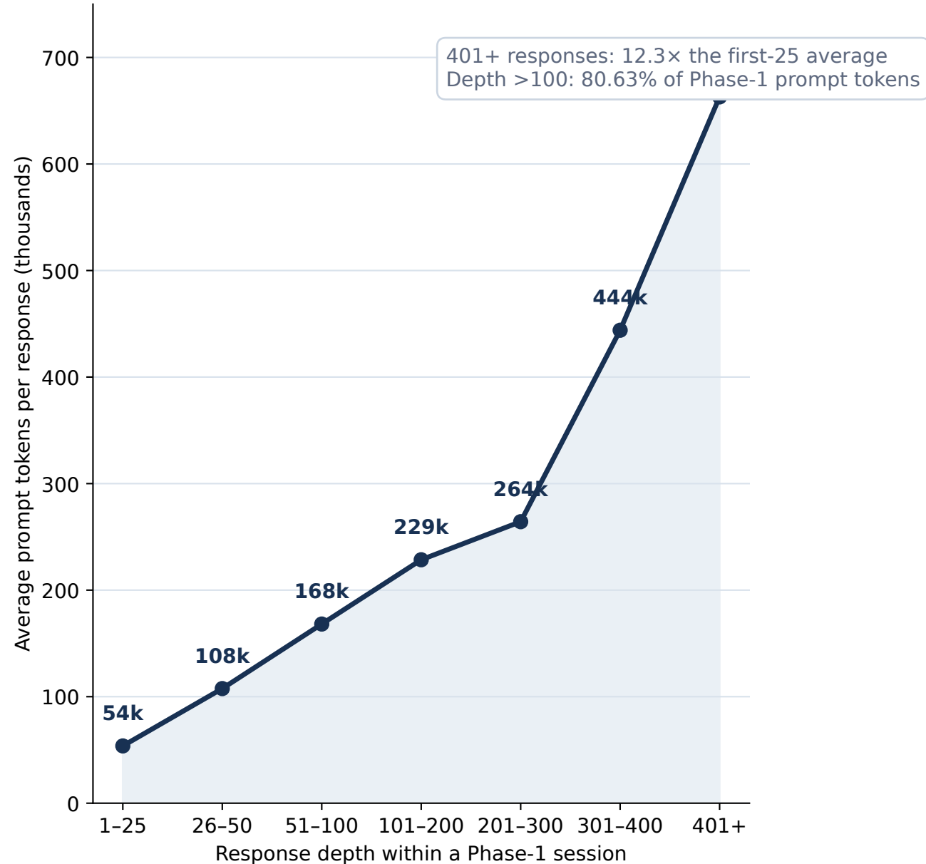
A. Long sessions replay increasingly large prompts
