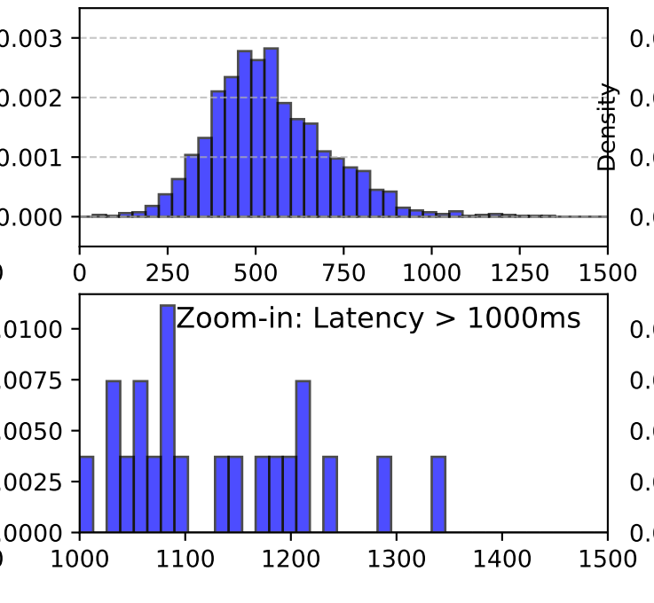
Nearest Neighbour
