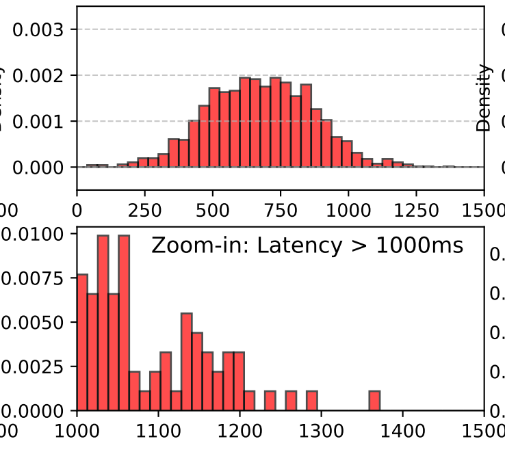
Chord
