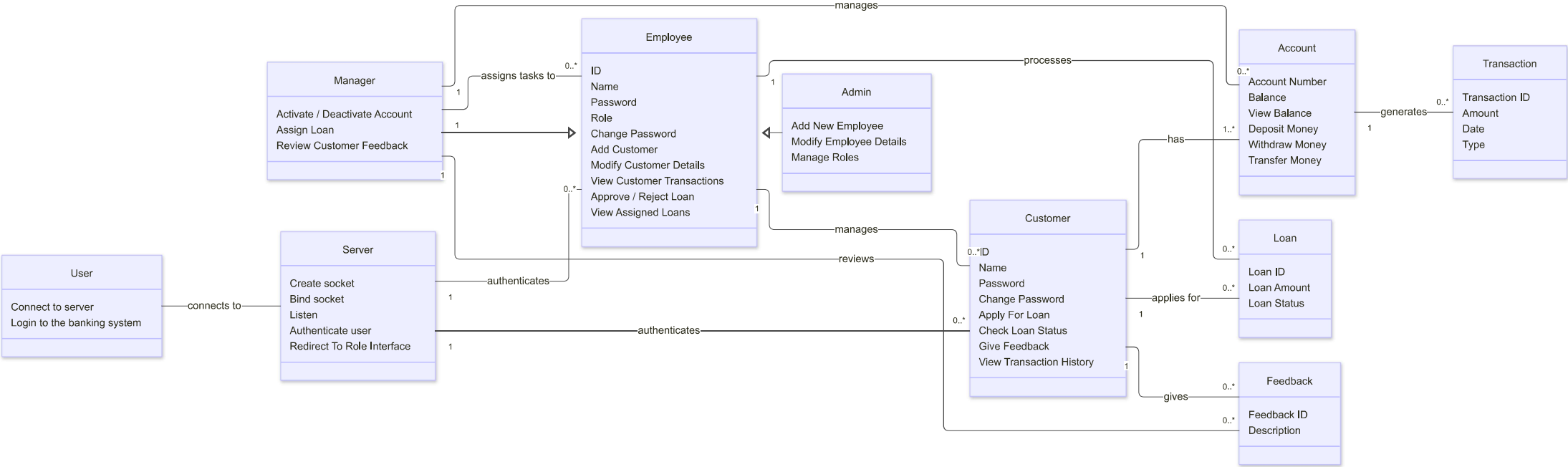
Banking Management System Class Diagram
