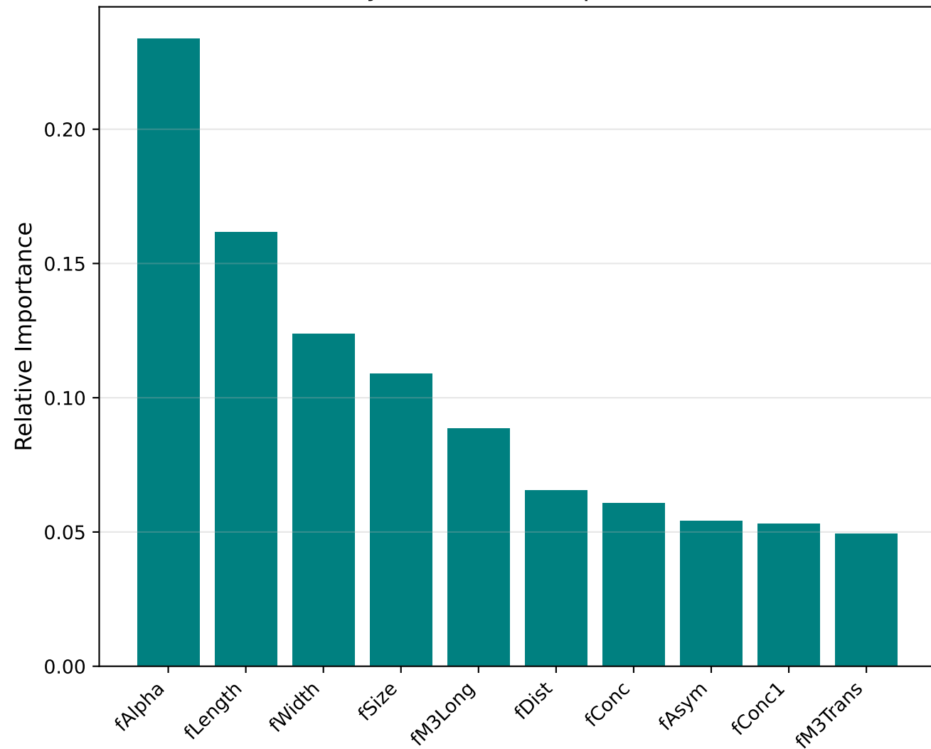
Physics Feature Importance
