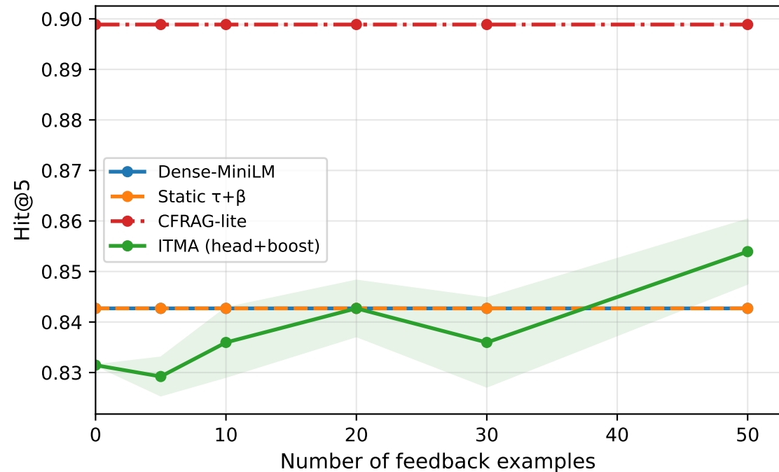
Cold-start adaptation curve
