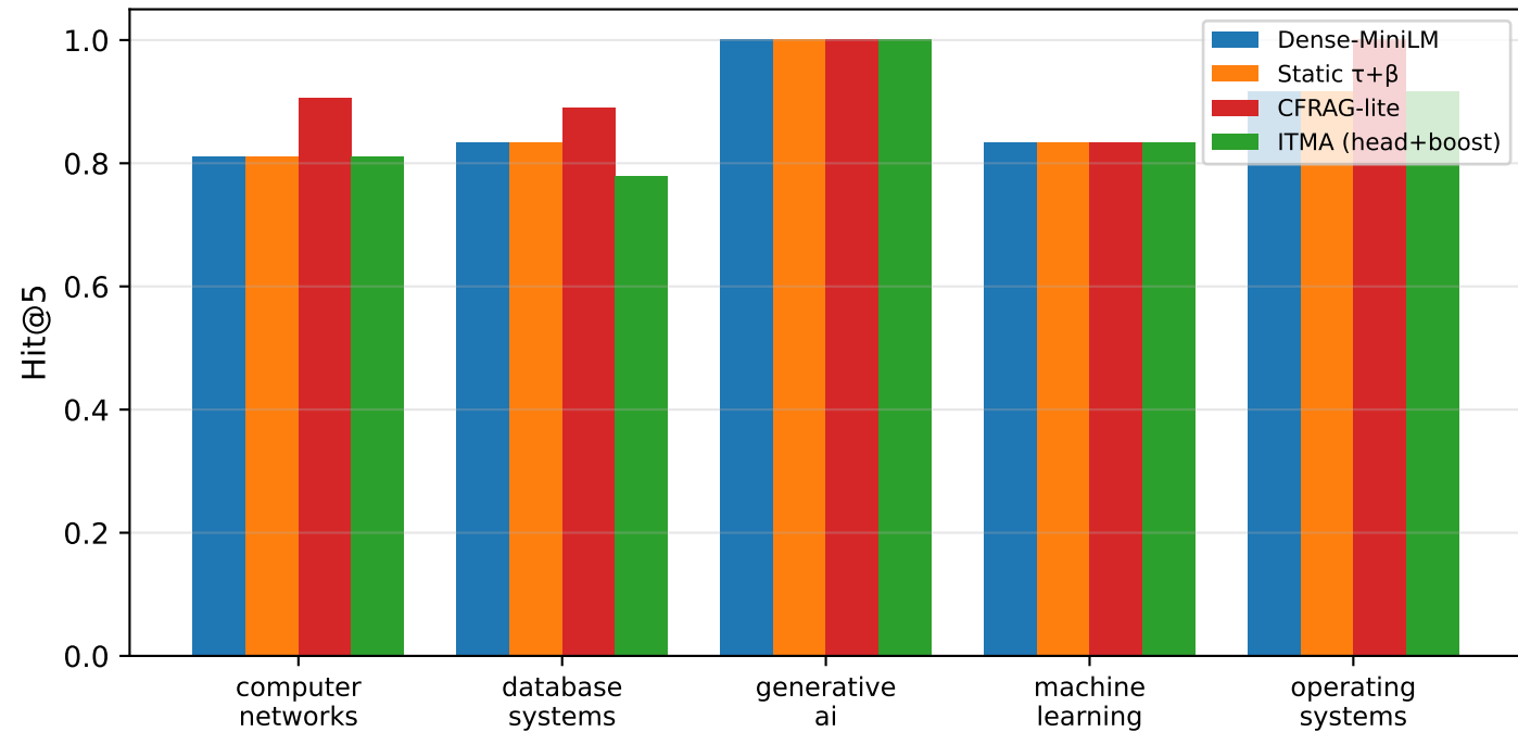
Per-domain retrieval performance
