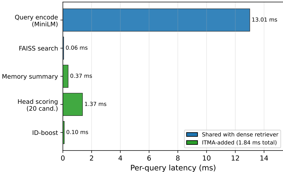
ITMA retrieval latency breakdown (CPU, |\mathcal{M}|=50 )
