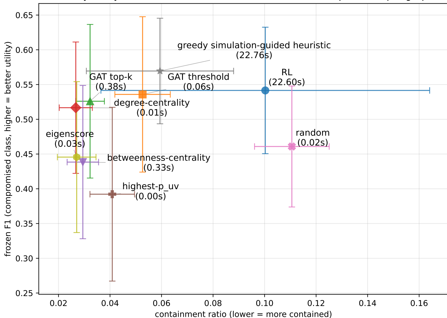
Security/utility trade-off across methods (label = mean compute cost per graph)
