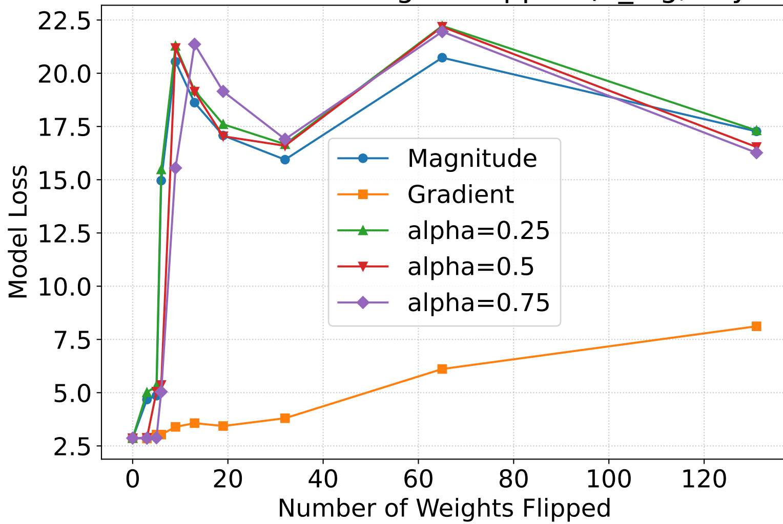
Loss vs. Number of Weights Flipped (A_log, Layer 47)
