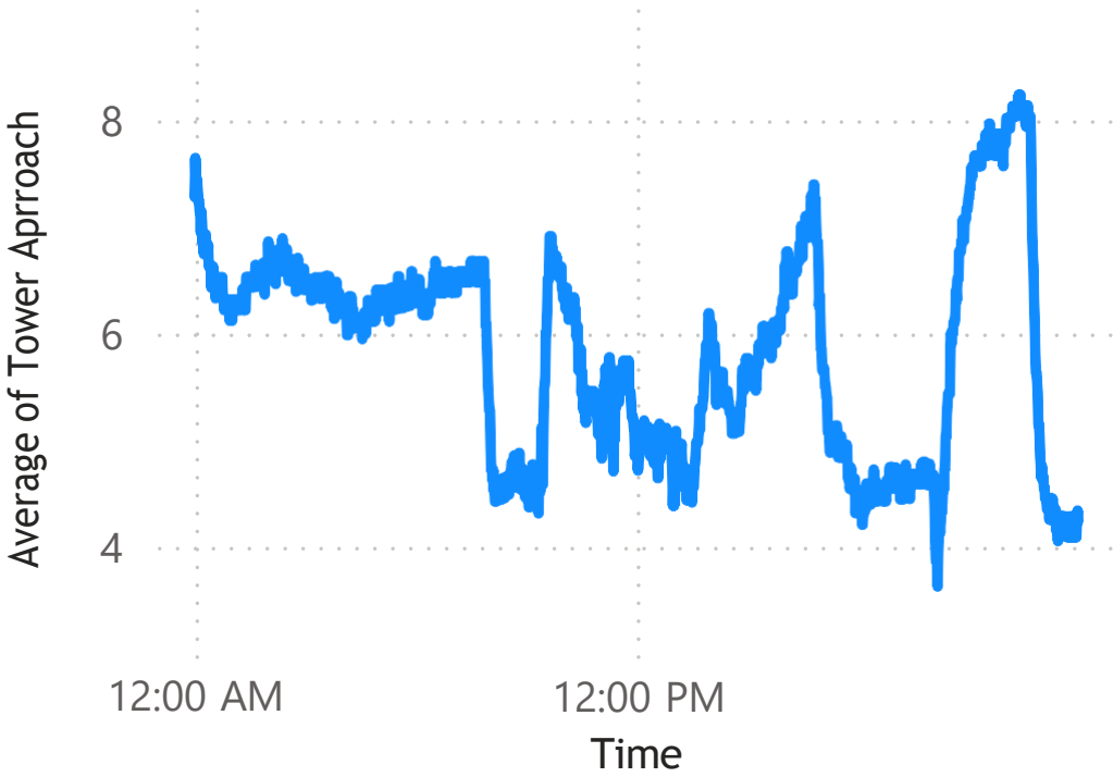
CT Approach
