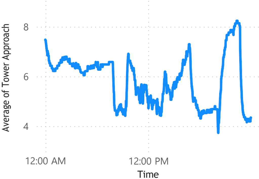
CT Approach
