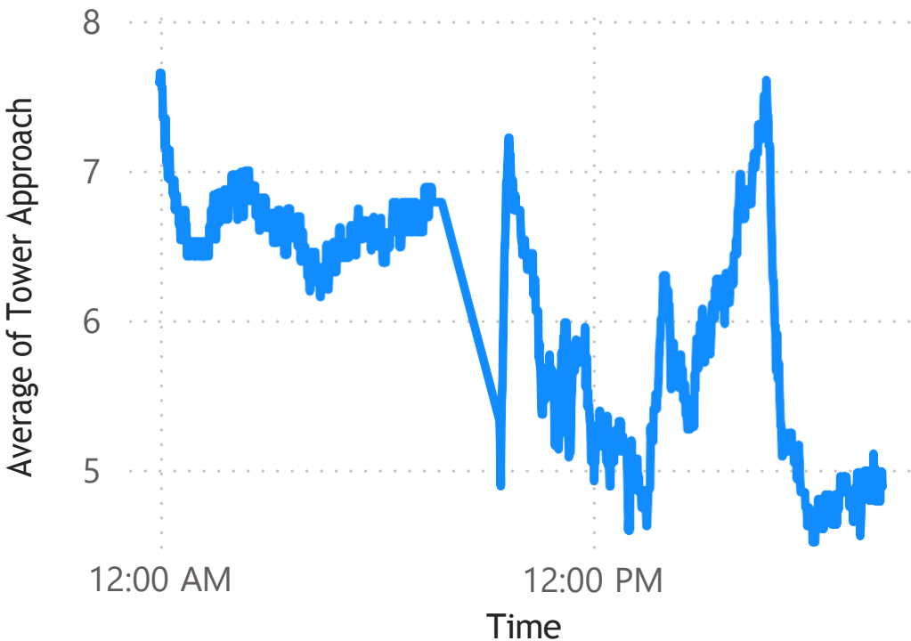
CT Approach
