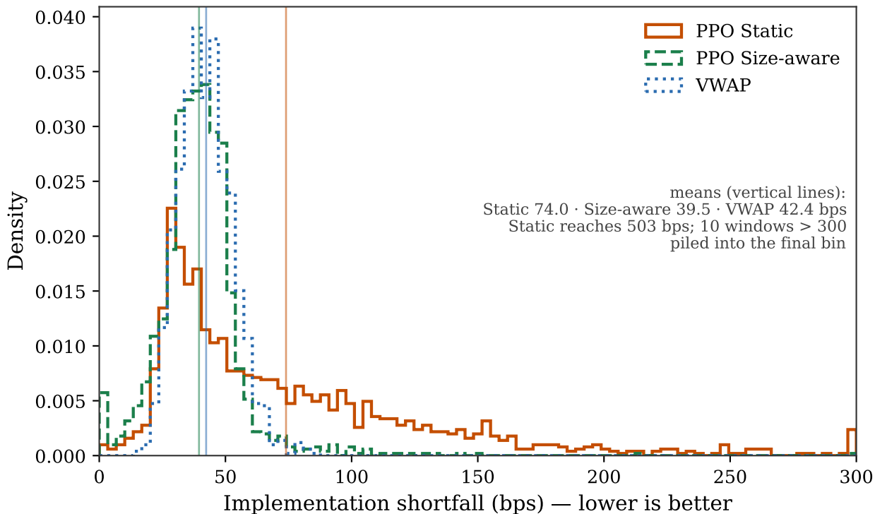
Distribution of execution shortfall across 1,500 test windows
