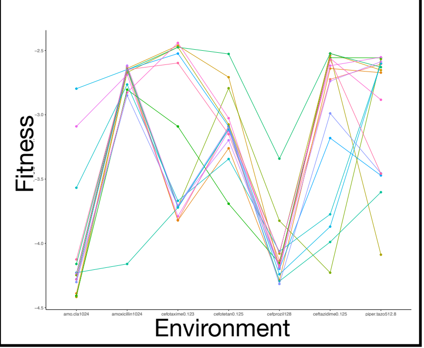
Reaction norms Genotype performance across environments
