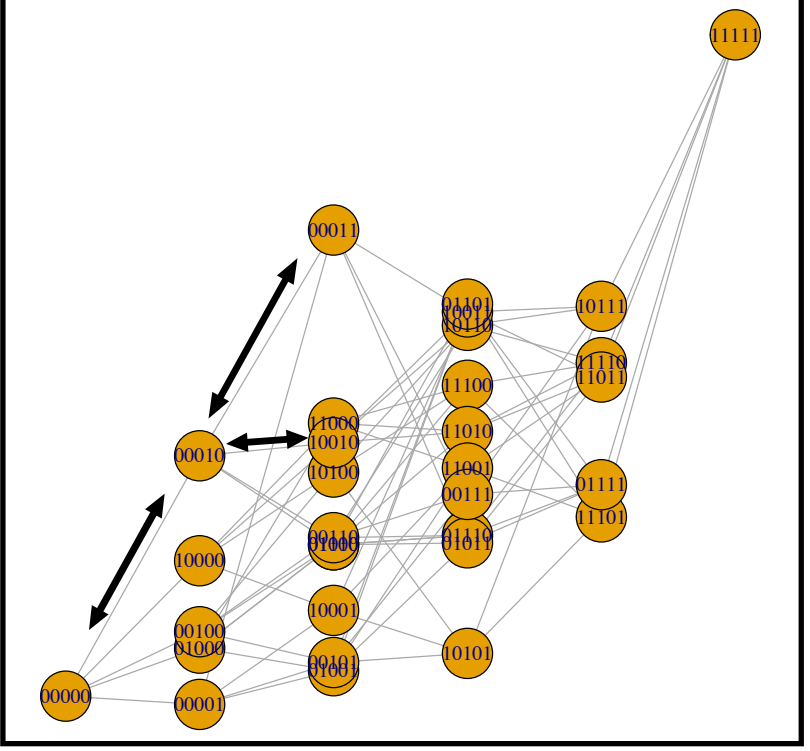
Features of trajectories change in mean/total within-path clonal interference across different environments
