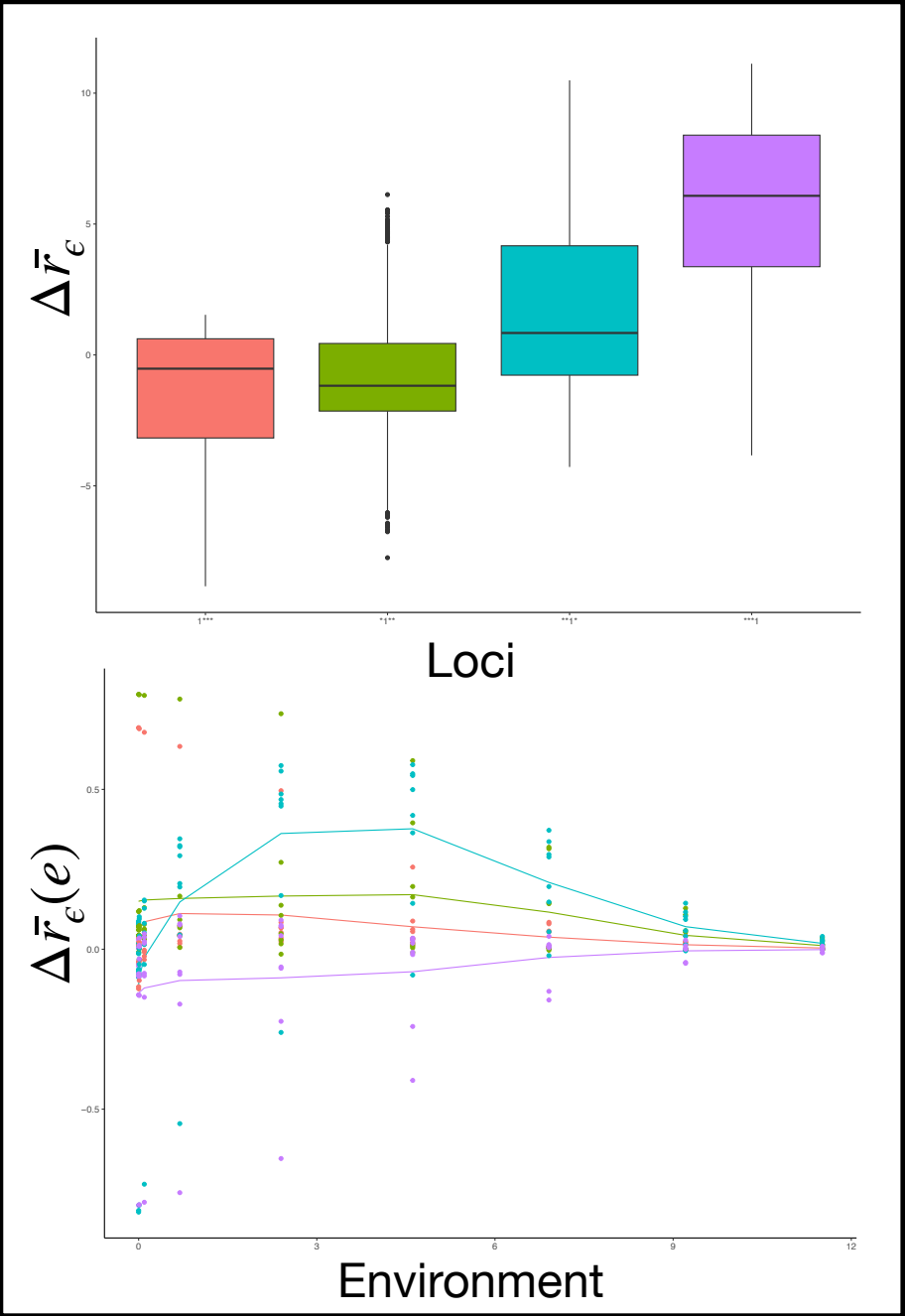
Robustness of loci robustness of loci across different genetic and environmental backgrounds
