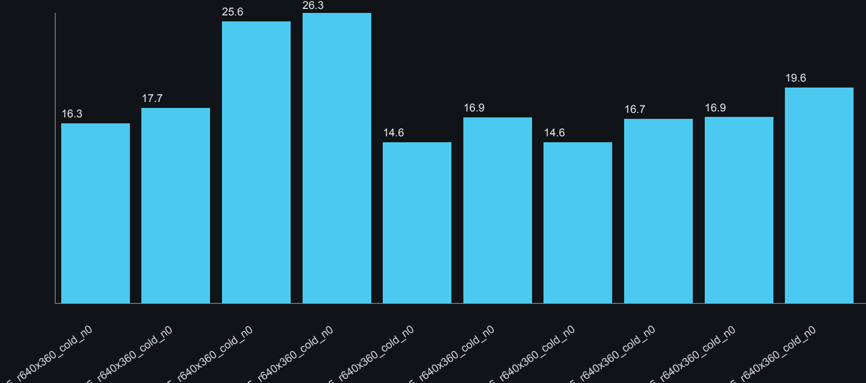
vulkan_gpu_measurements Semantic Utility per CPU Millisecond
