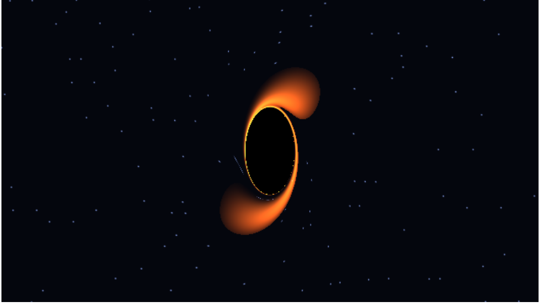
Figure 2: Checked Schwarzschild thin-disk frame. Captured rays form the central shadow; disk placement derives from an RK4 deflection lookup, with a heuristic brightness model.
