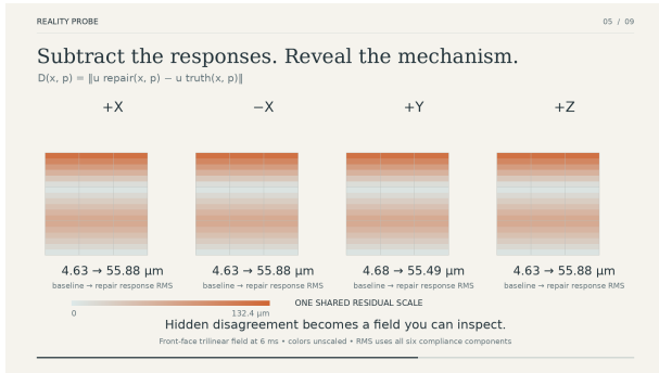
Fig. 6. Spatial residual field for the same visualization case. The field localizes disagreement between responses; it is not itself the acceptance statistic.
