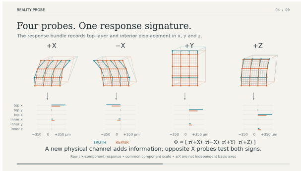
Fig. 5. Four-direction force-response fingerprint for one frozen visualization case. The response bundle records top-layer and interior displacement under the four load directions.
