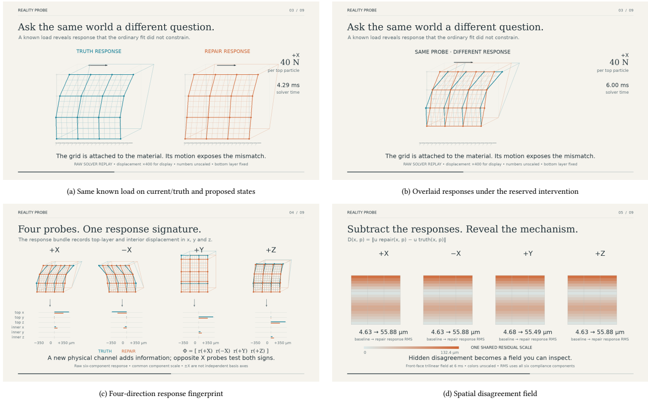
Fig. 4. Concrete force-compliance example from the controlled synthetic study. A known +x load of 40 N per top-layer particle is applied to the current/truth and proposed material states; the displayed deformation is magnified 400 \times only for visibility. Panels (a–b) show the simulated physical states and their response overlay, while (c–d) expose the multi-direction response and where the two states disagree. Quantitative acceptance uses the unscaled responses and uncertainty model, not the display magnification or the residual image by itself.
