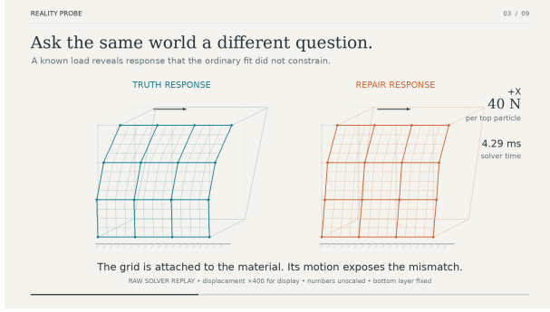
Fig. 4. The same known +x force is applied to truth and proposed models. Deformation is magnified 400 \times for visualization only; all quantitative values use unscaled displacement.
