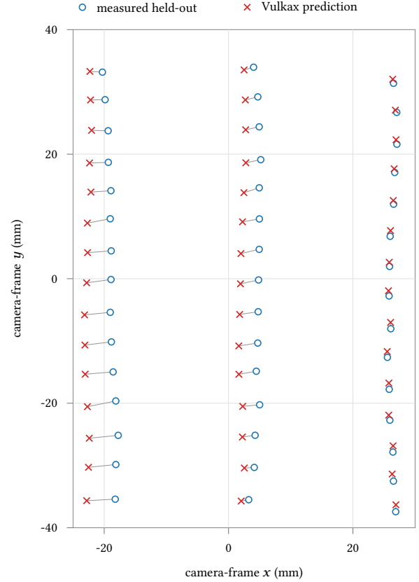
Fig. 3. Held-out DOT C2 measured-versus-predicted geometry at t = 0.167 s. Circles are measured correspondences, crosses are predictions, and connecting segments are true-scale residuals.
