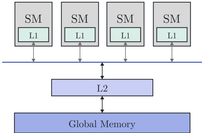
Figure 1: Simplified GPU memory hierarchy.
