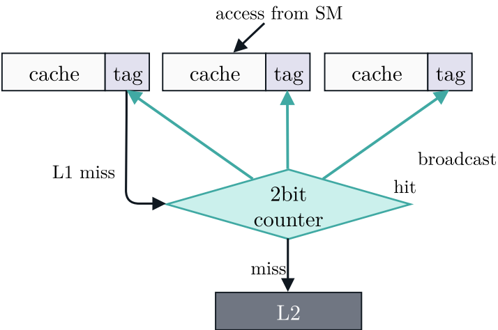
(b) CCD [18] cache sharing
