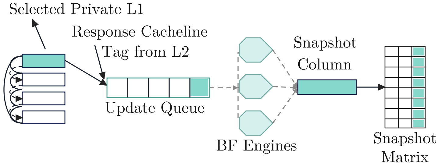
Figure 9: Refresh path of C2P-Cache.
