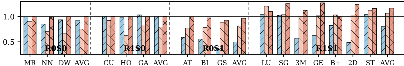
Normalized IPC
