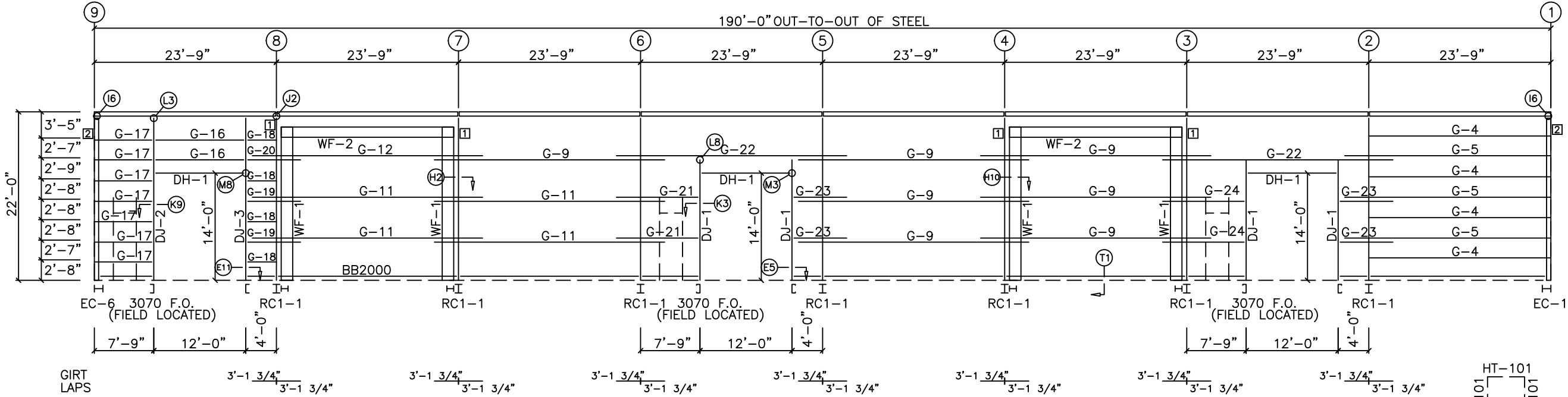
BACK SIDEWALL FRAMING: LINE A
