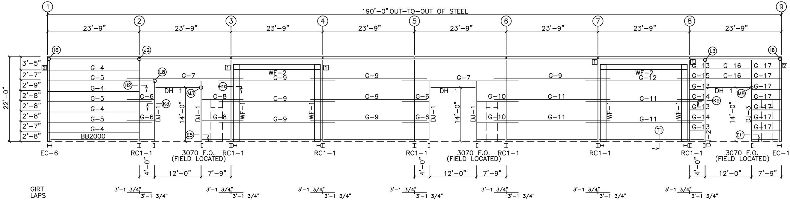
FRONT SIDEWALL FRAMING: LINE F
