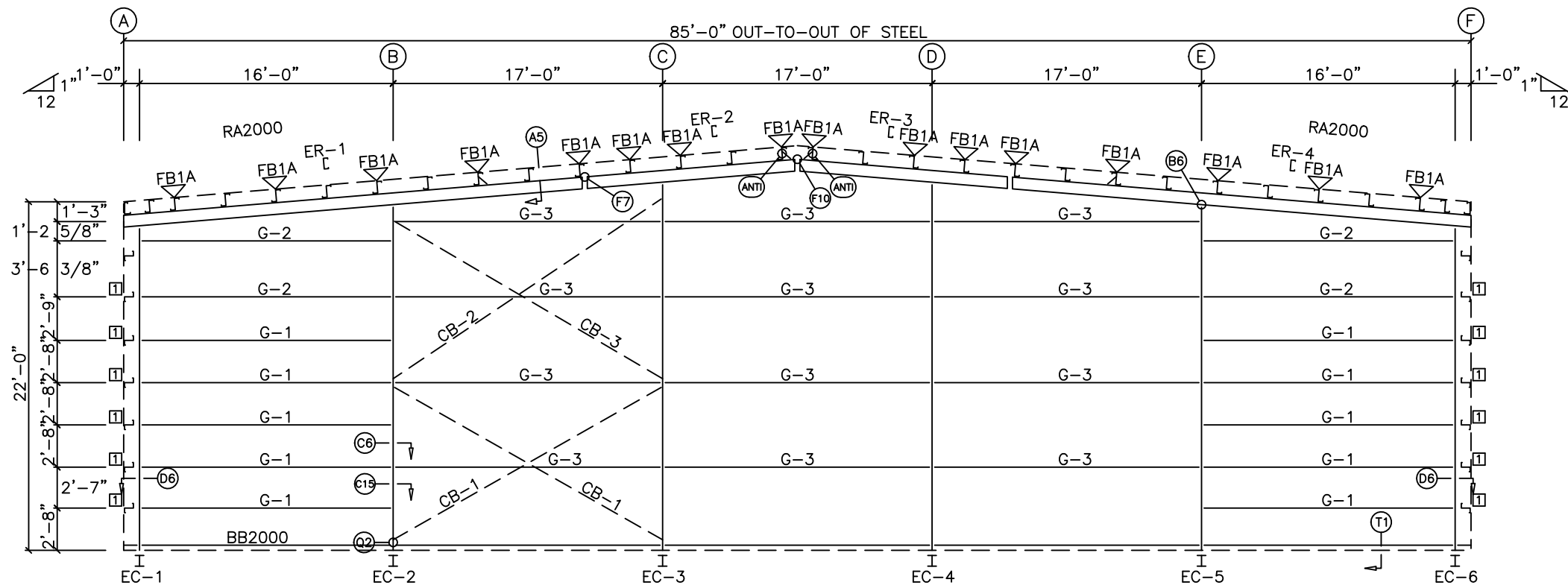
ENDWALL FRAMING: LINE 1
