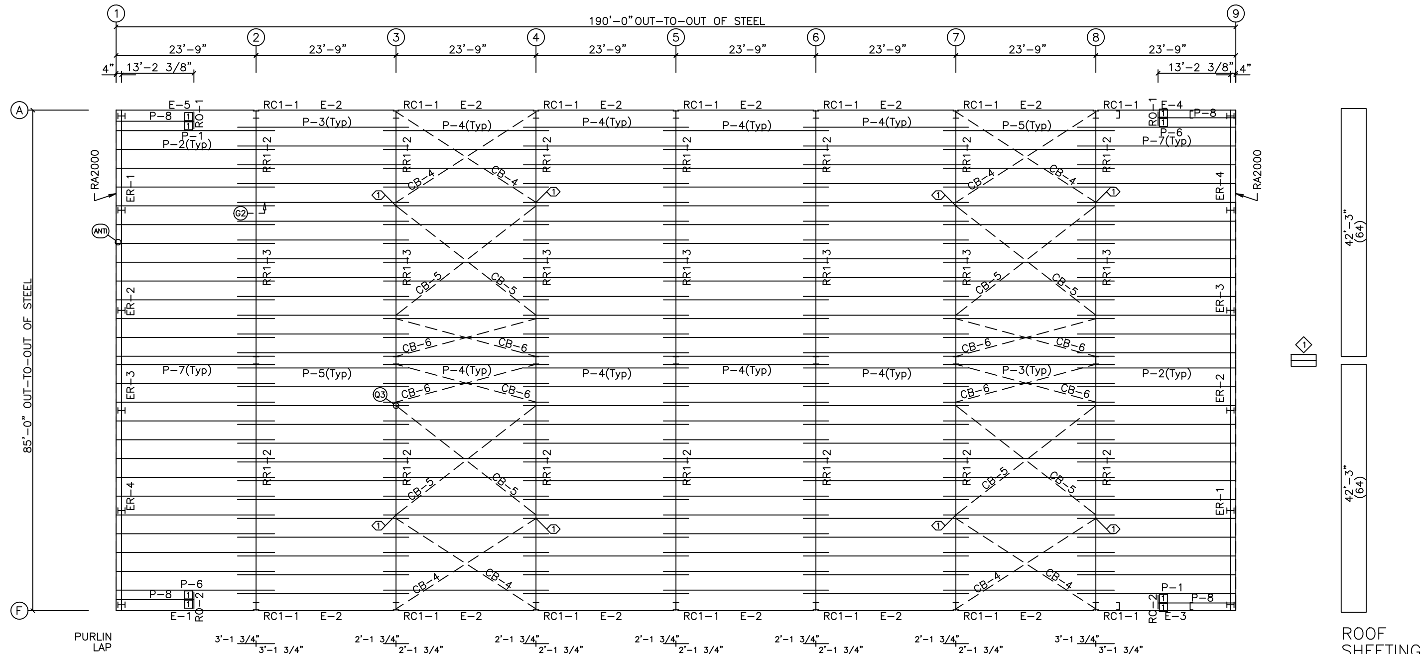
ROOF FRAMING PLAN
