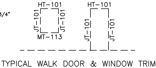
TYPICAL WALK DOOR & WINDOW TRIM
