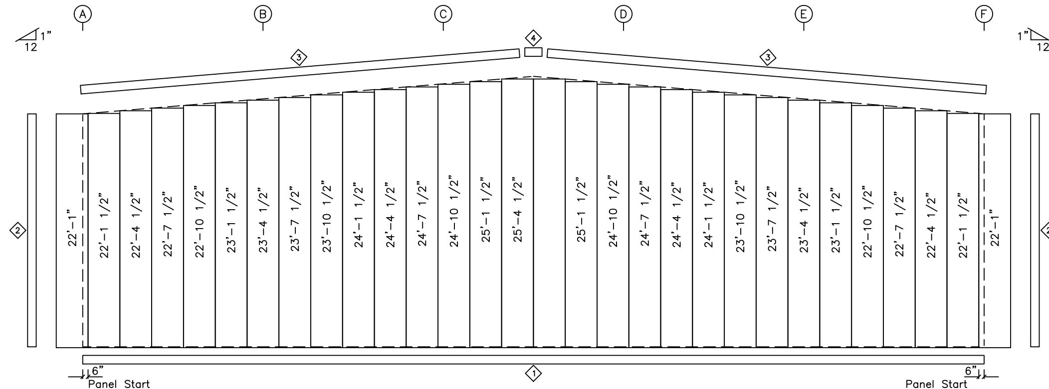
ENDWALL SHEETING & TRIM: LINE 1
