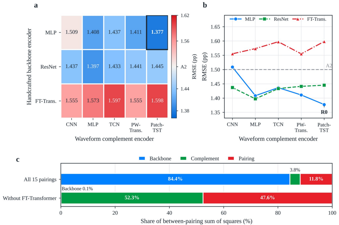
517 Fig. 3. Main effects and pairing dependence in the encoder matrix. (a) Cell-macro RMSE of 518 the 15 pairings; the diverging scale is centred on the backbone-only model A2 (1.500 pp), 519 blue denoting lower and red higher error; the frame marks R0. (b) Interaction plot; non- 520 parallel lines indicate pairing dependence; the dashed line marks A2. (c) Share of the 521 between-pairing sum of squares due to backbone, complement and pairing for all 15 pairings 522
