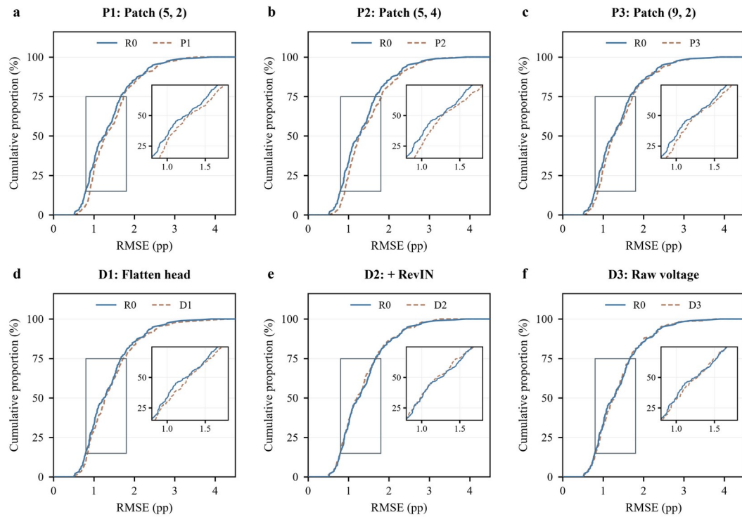
270 271 Fig. S1. Cumulative error distributions of the waveform-branch design variants. (a–c) Patch 272 configurations P1 (5, 2), P2 (5, 4) and P3 (9, 2) versus R0 (9, 4); (d–f) adaptation ablations 273 D1 (flatten head), D2 (with RevIN) and D3 (raw voltage). Solid blue, R0; dashed brown, 274 variant. Each curve contains the 192 cell \times seed RMSEs (not 192 independent cells); insets 275 magnify RMSE 0.8–1.8 pp and cumulative proportion 15–75%. Cell-level tests are given in 276 Table 8.
