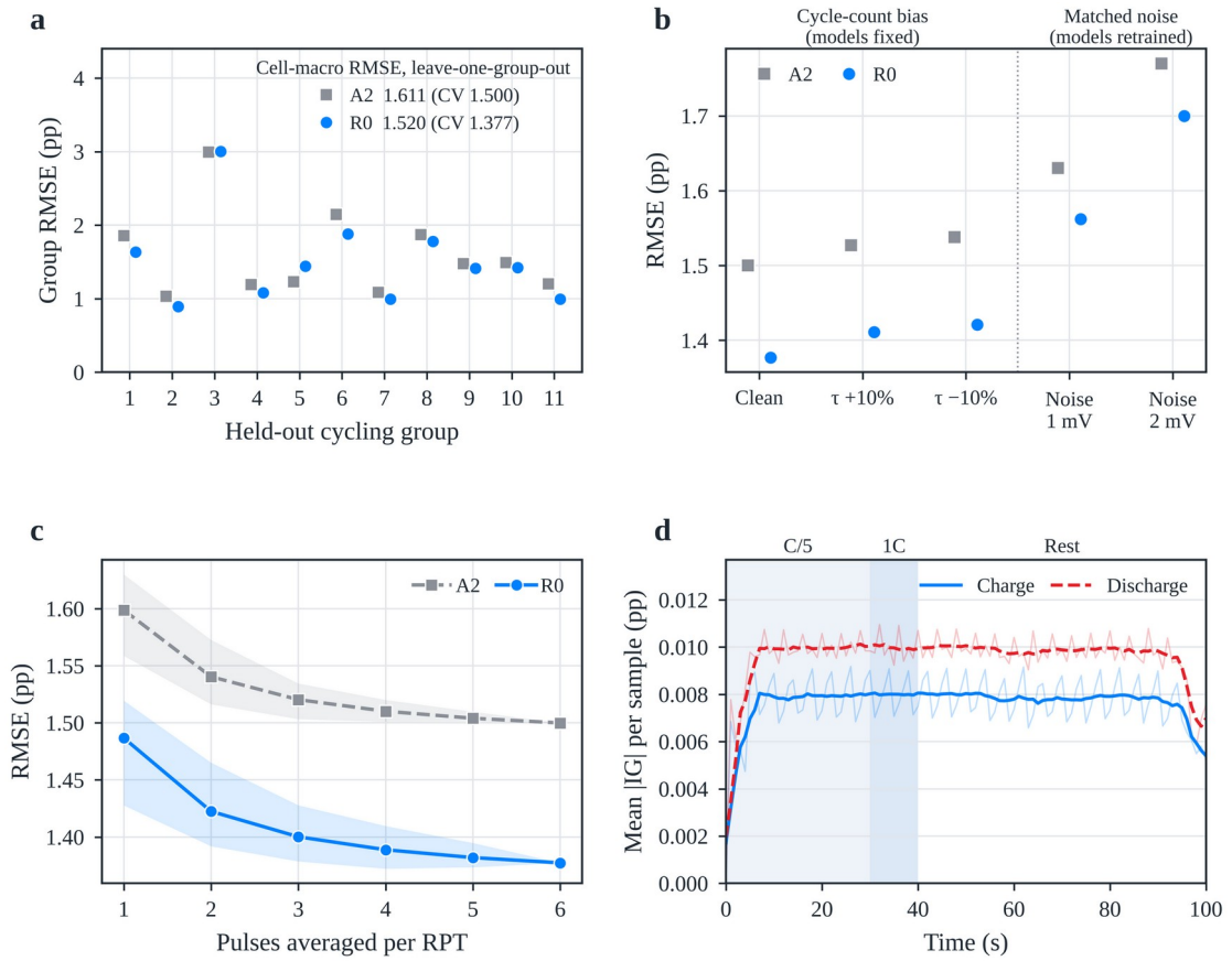
Fig. 7. Generalisation, robustness and attribution. (a) Group-mean RMSE when each cycling group is held out (leave-one-group-out); the legend gives the cell-macro RMSE under leave-one-group-out and, in parentheses, under five-fold cell-disjoint validation. (b) RMSE with a \pm 10\% bias of the test cycle count (models fixed) and with matched Gaussian voltage noise in training and test data (models retrained). (c) RMSE versus the number of pulses averaged per RPT; lines show the mean over all condition combinations and bands their range. (d) Mean absolute integrated-gradient attribution of R0 per waveform sample for charge (solid) and discharge (dashed) pulses, averaged over test records, folds and seeds; shading marks the pulse segments.
