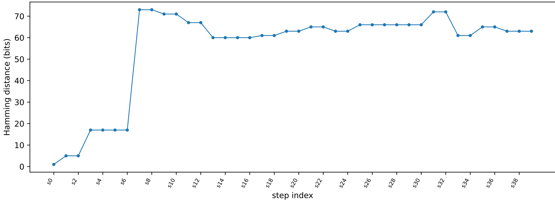
Q1 part c custom mix (P vs P', key fixed)
