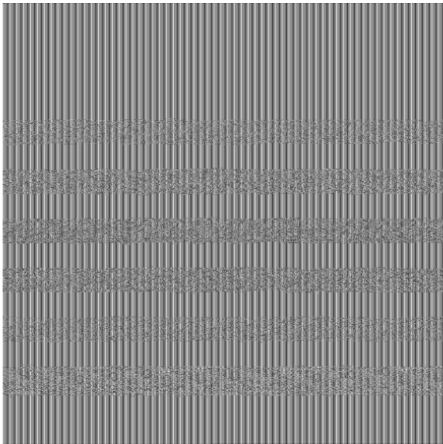
ECB ciphertext bytes (pixel body)
