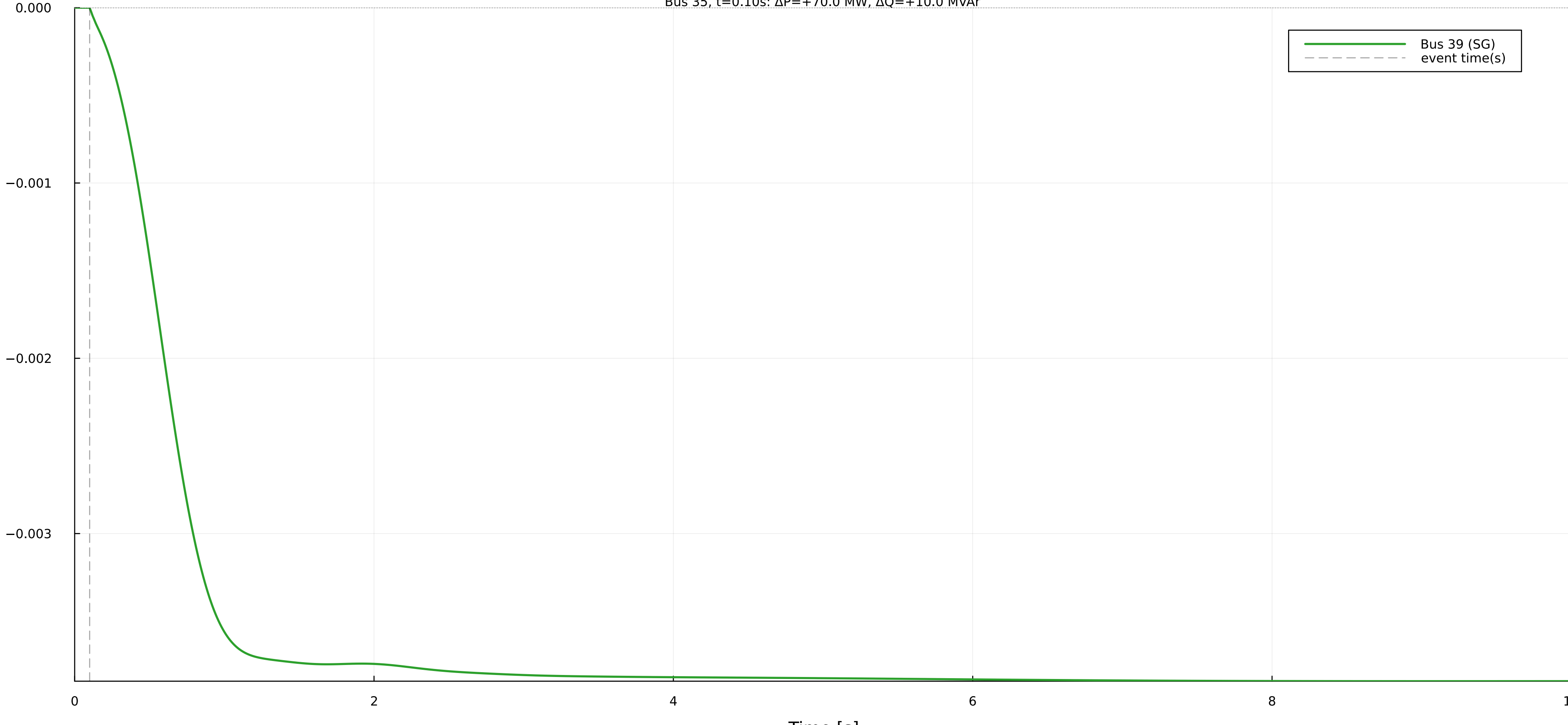
Frequency deviation at bus 39 Bus 35, t=0.10s: \Delta P=+70.0 MW, \Delta Q=+10.0 MVar
