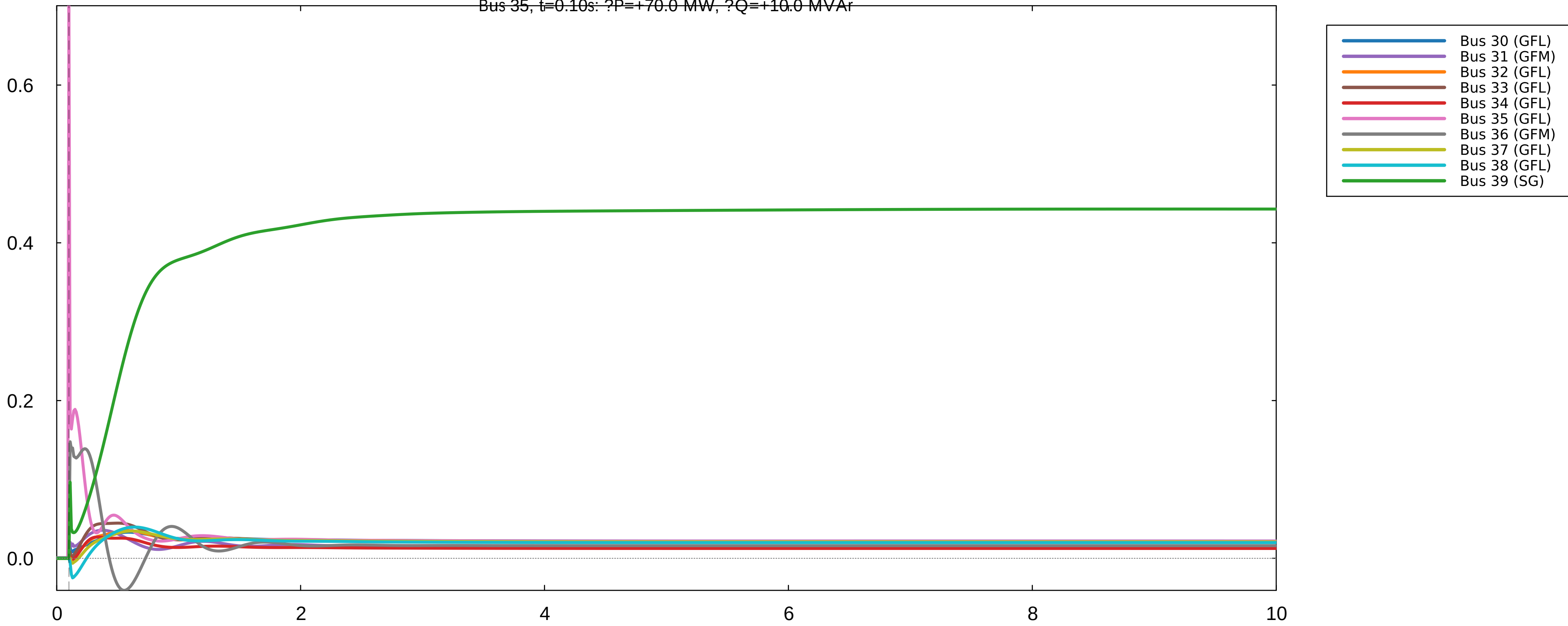
Reconstructed network active - power deviation from Ybus
