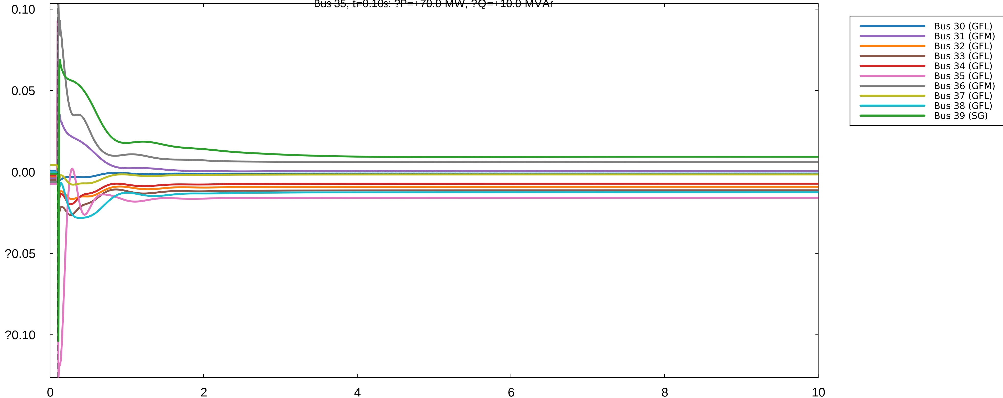
Reconstructed network reactive - power deviation from Ybus
