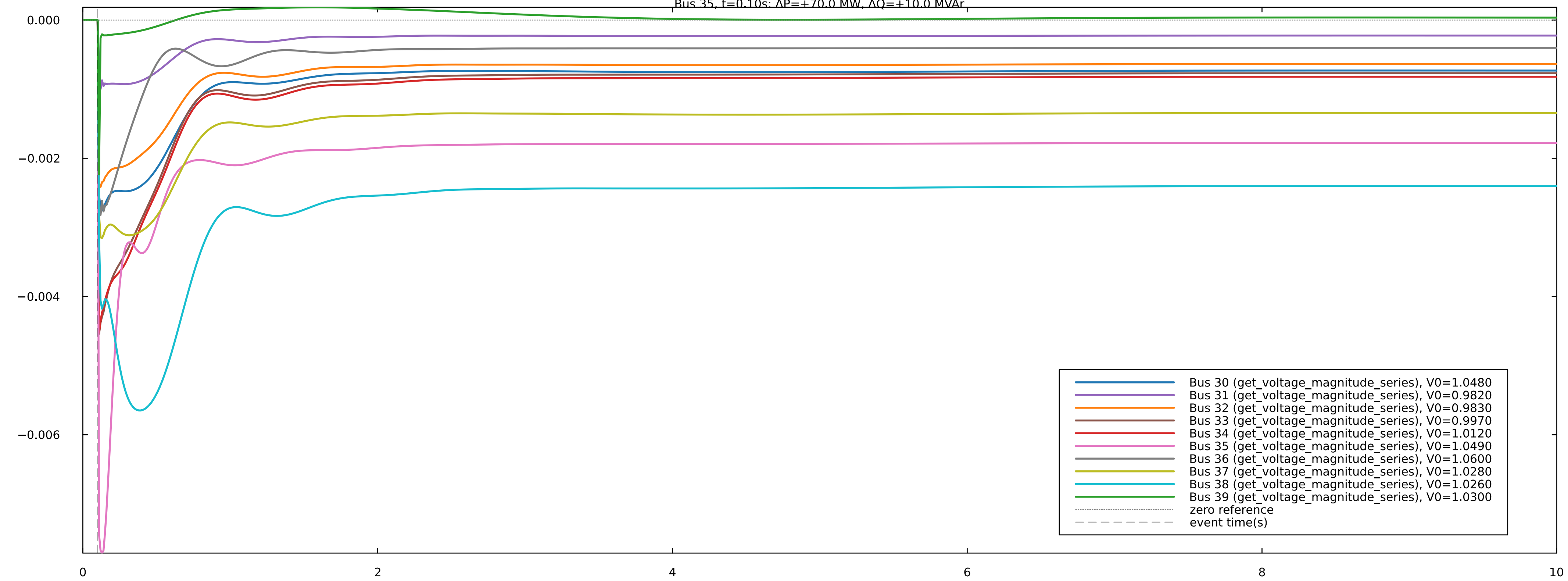
Bus voltage-magnitude deviations from initial value Bus 35, t=0.10s: \Delta P=+70.0 MW, \Delta Q=+10.0 MVar
