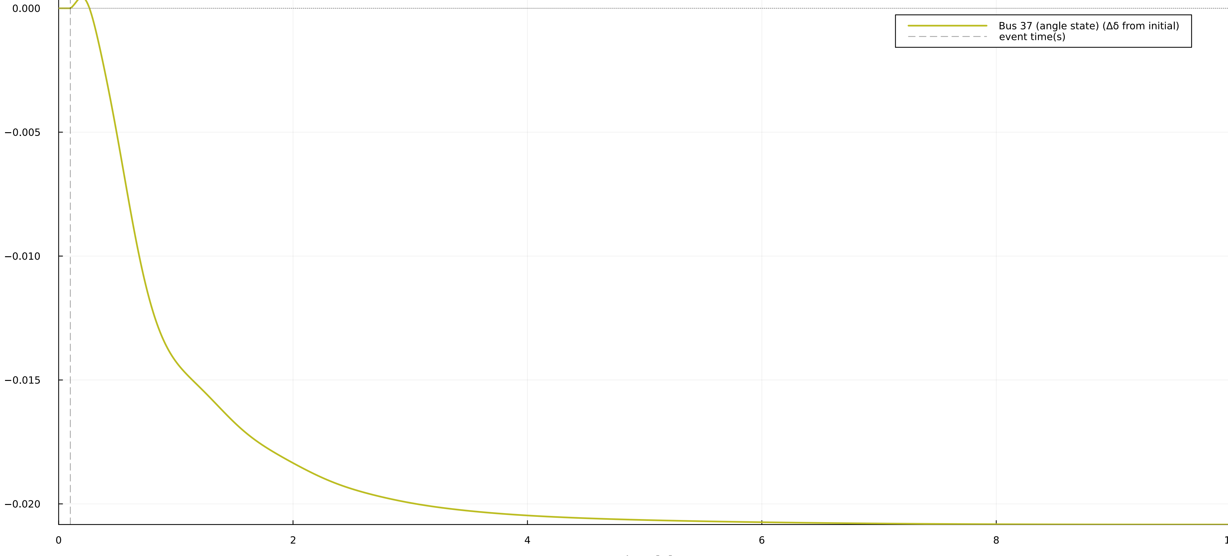
Rotor/angle deviation at bus 37 Bus 35, t=0.10s: \Delta P=+70.0 MW, \Delta Q=+10.0 MVar
