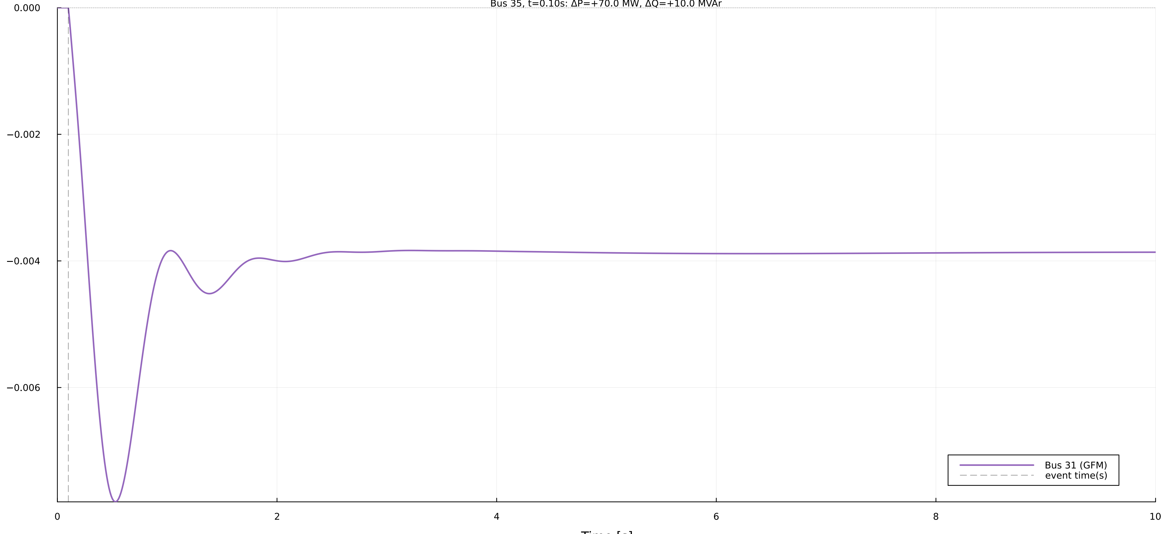
Frequency deviation at bus 31 Bus 35, t=0.10s: \Delta P=+70.0 MW, \Delta Q=+10.0 MVar
