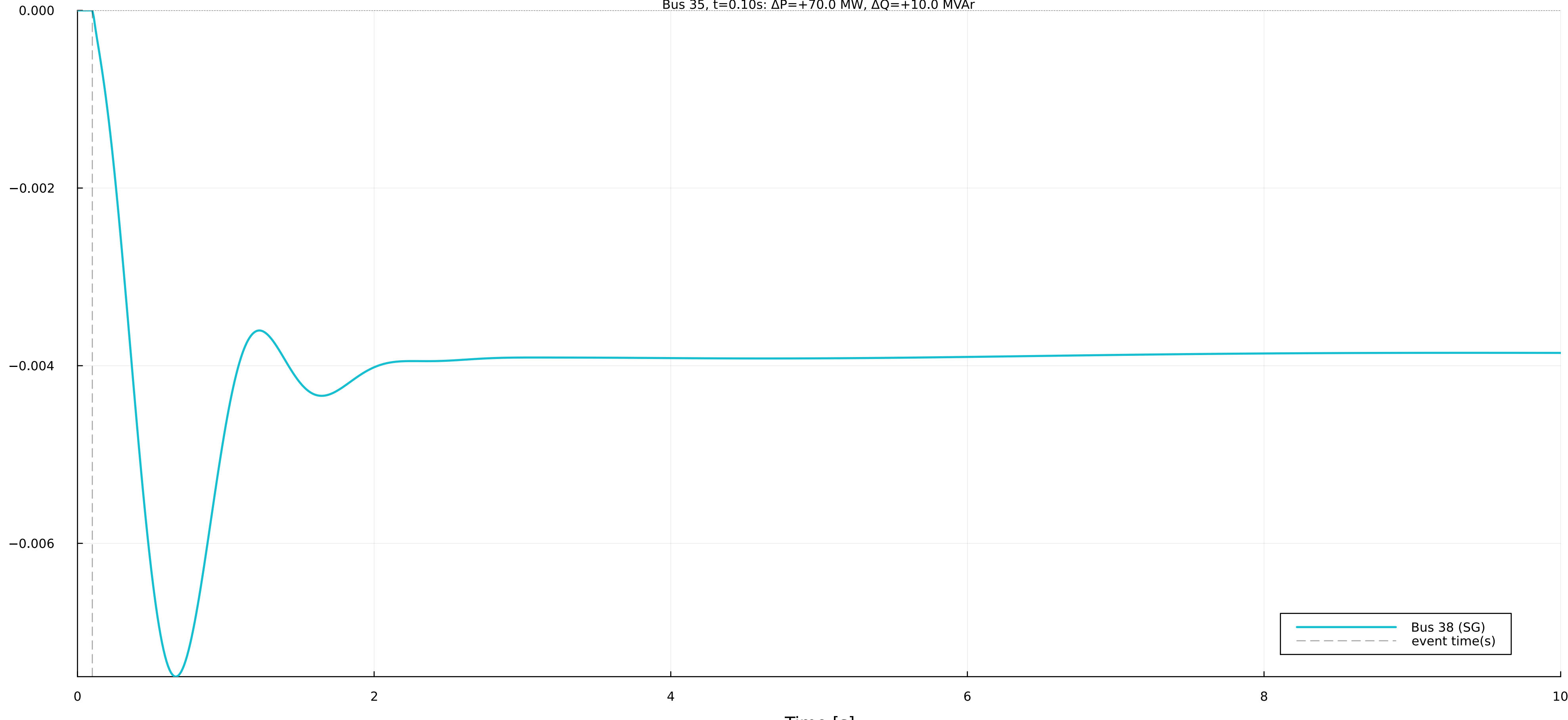
Frequency deviation at bus 38 Bus 35, t=0.10s: \Delta P=+70.0 MW, \Delta Q=+10.0 MVar
