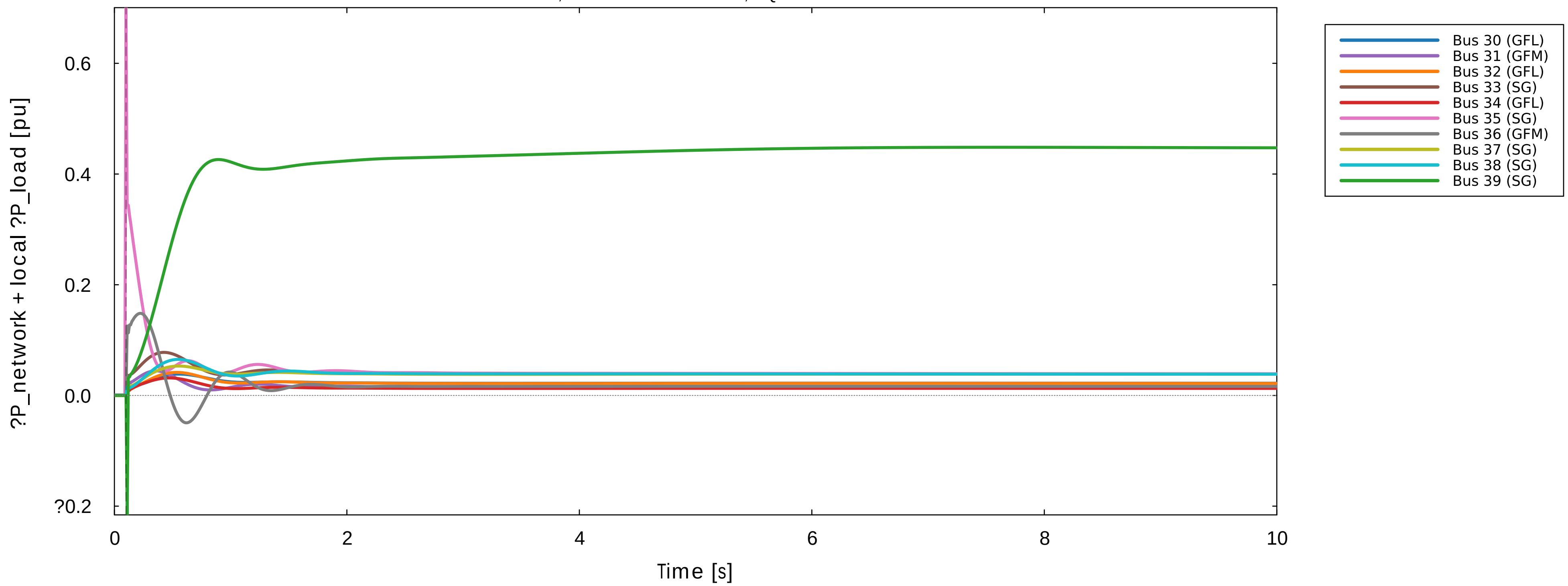
Reconstructed network active - power deviation from Ybus Bus 35, t=0.10s: ?P=+70.0 MW, ?Q=+10.0 MVar
