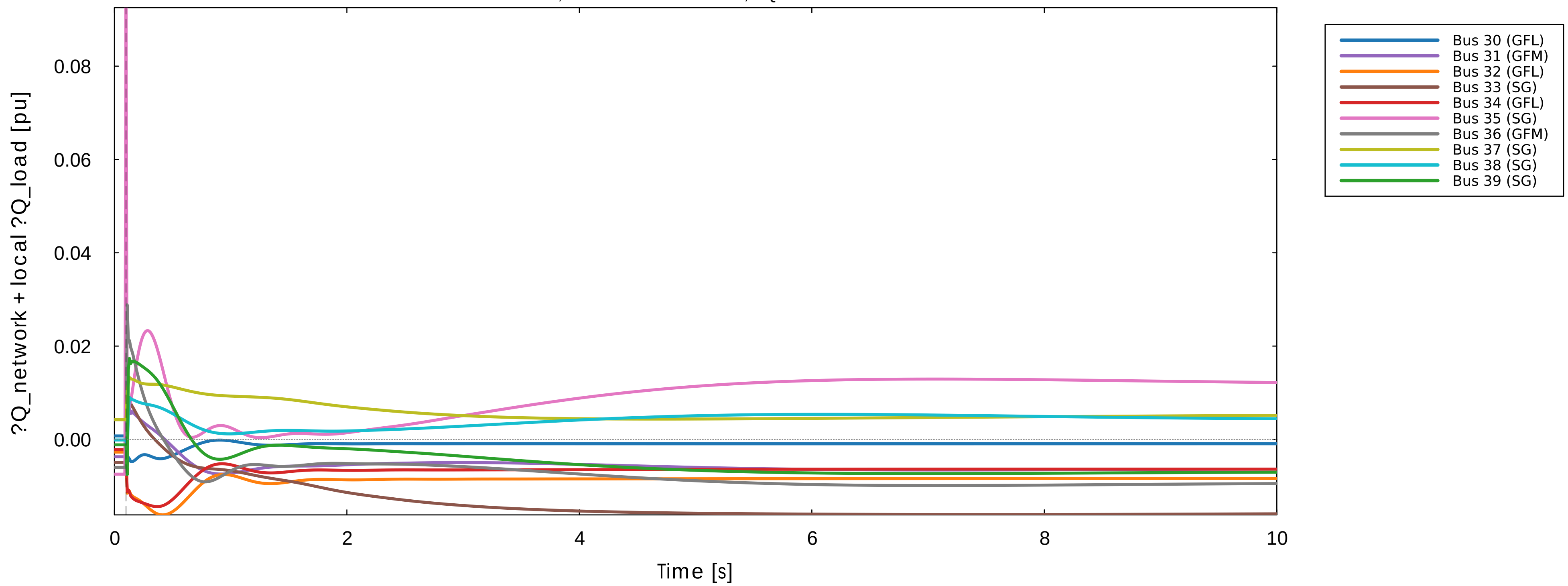
Reconstructed network reactive - power deviation from Ybus Bus 35, t=0.10s: ?P=+70.0 MW, ?Q=+10.0 MVar
