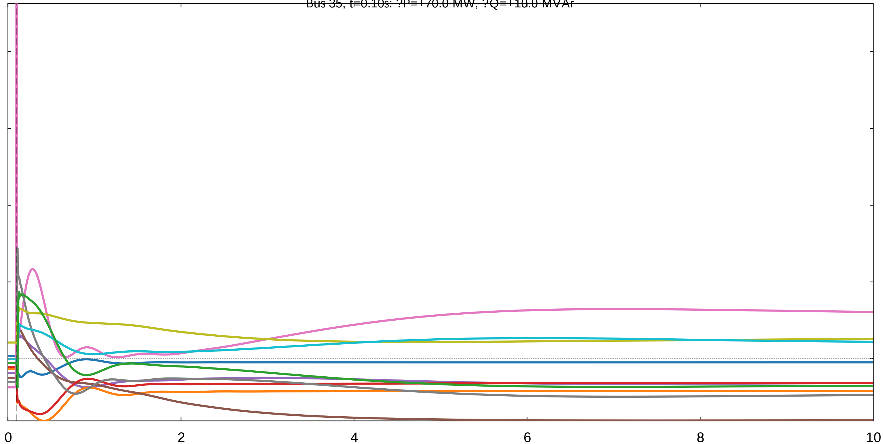
Reconstructed network reactive - power deviation from Ybus
