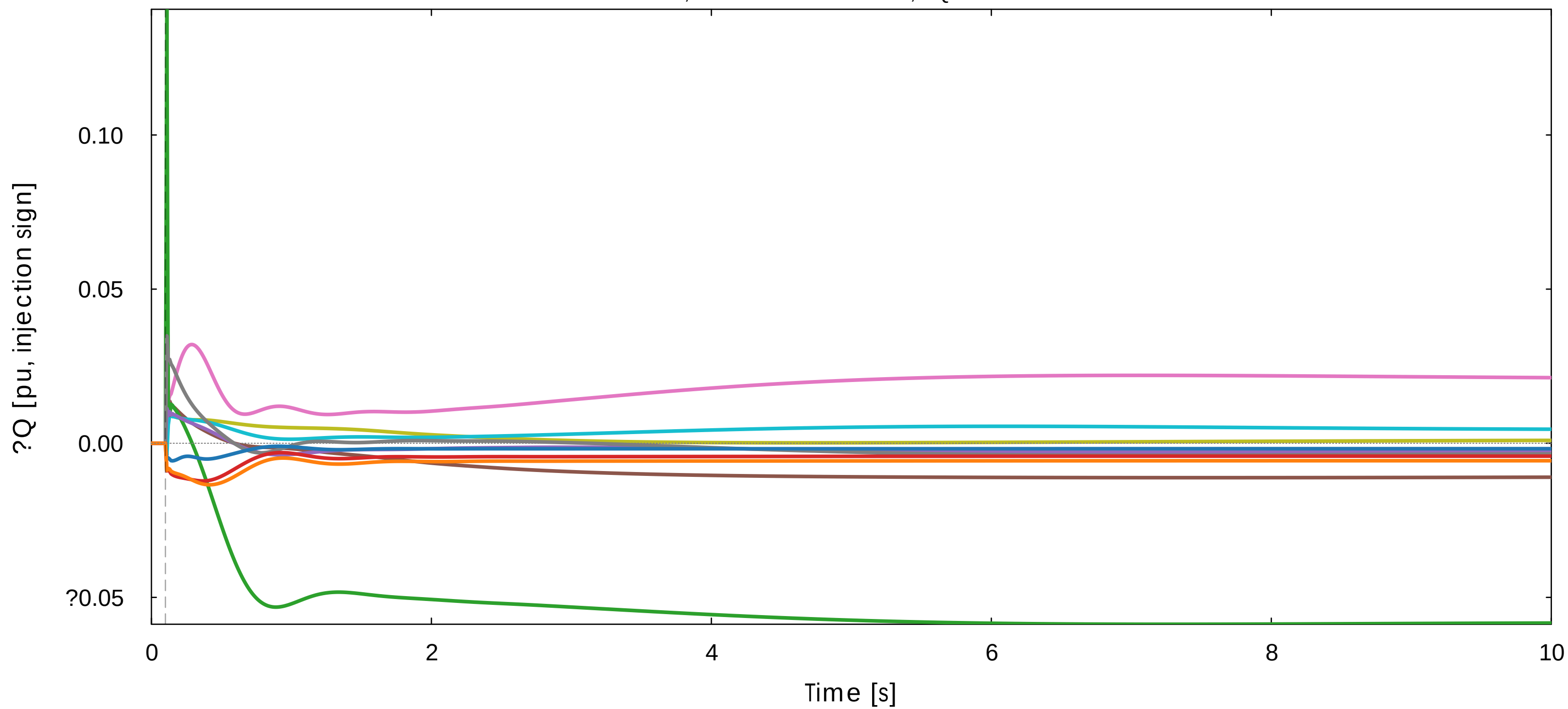
Terminal reactive - power deviation (device electrical output) Bus 35, t=0.10s: ?P=+70.0 MW, ?Q=+10.0 MVA
