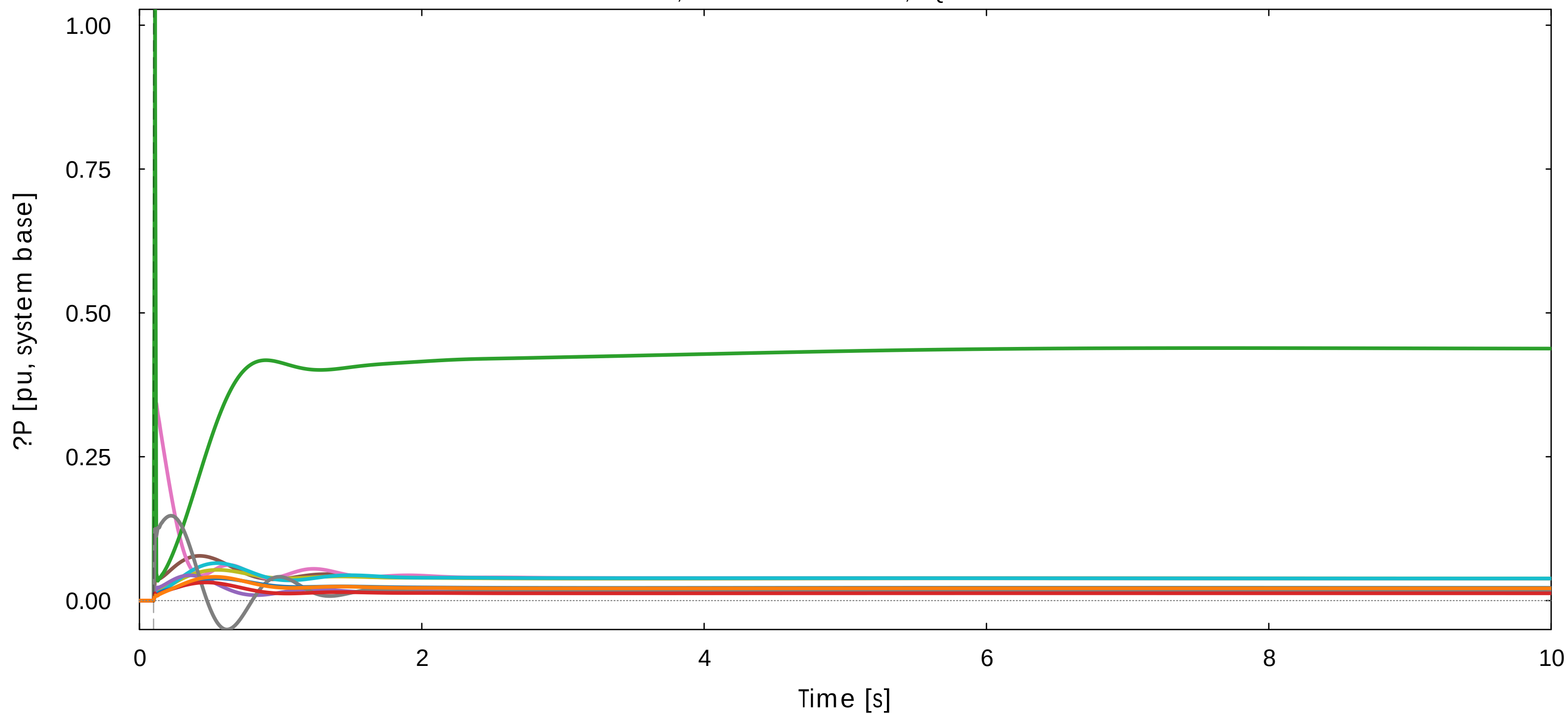
Terminal active - power deviation (device electrical output) Bus 35, t=0.10s: ?P=+70.0 MW, ?Q=+10.0 MVA
