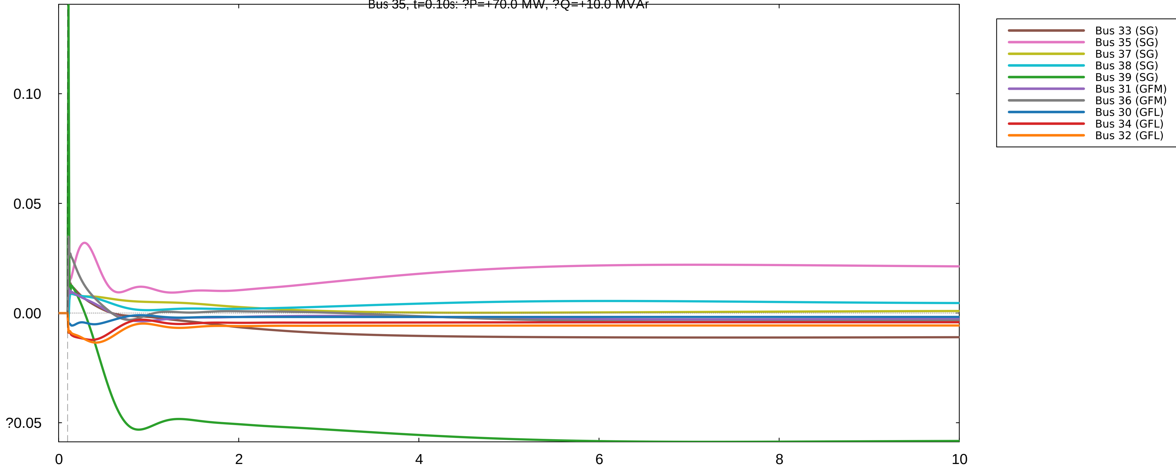
Terminal reactive - power deviation (device electrical output)
