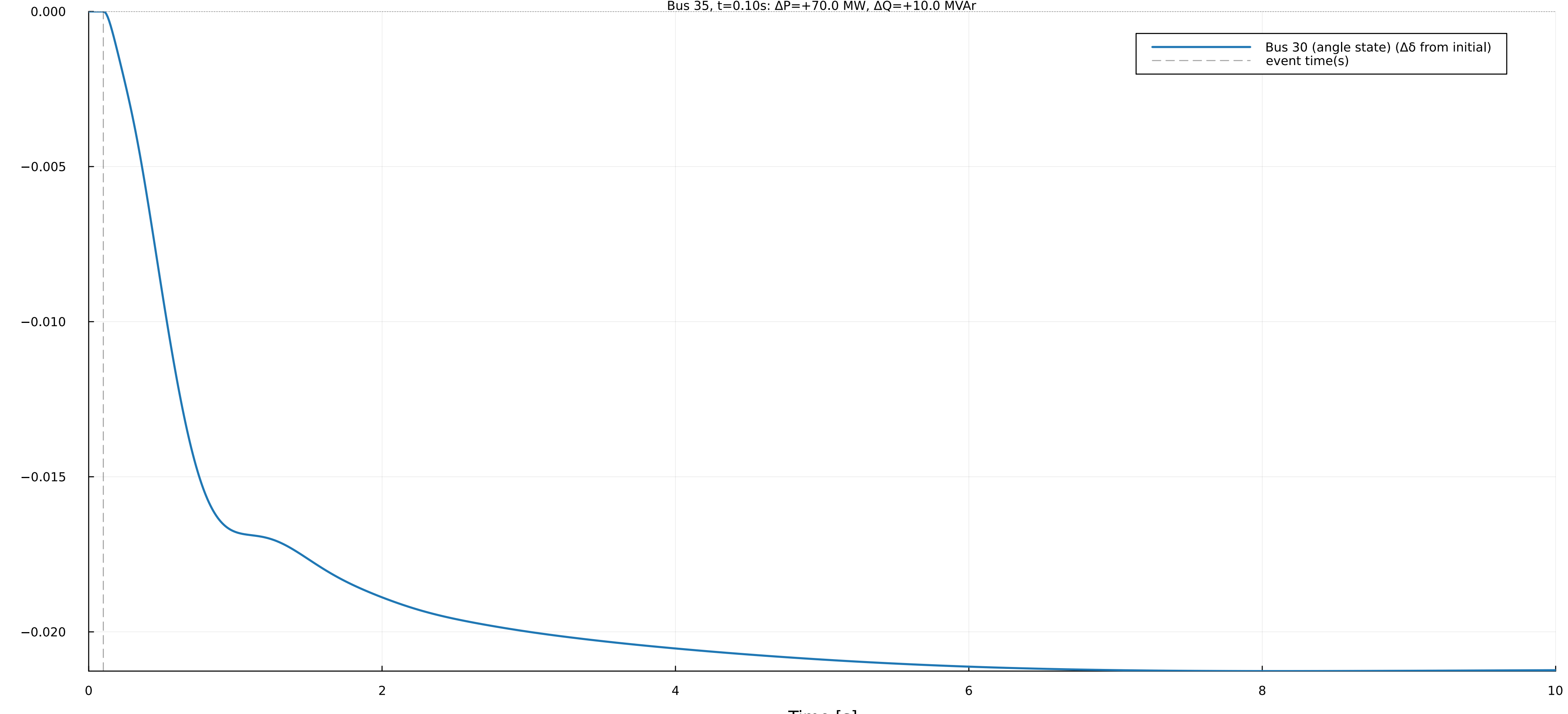
Rotor/angle deviation at bus 30 Bus 35, t=0.10s: \Delta P=+70.0 MW, \Delta Q=+10.0 MVar
