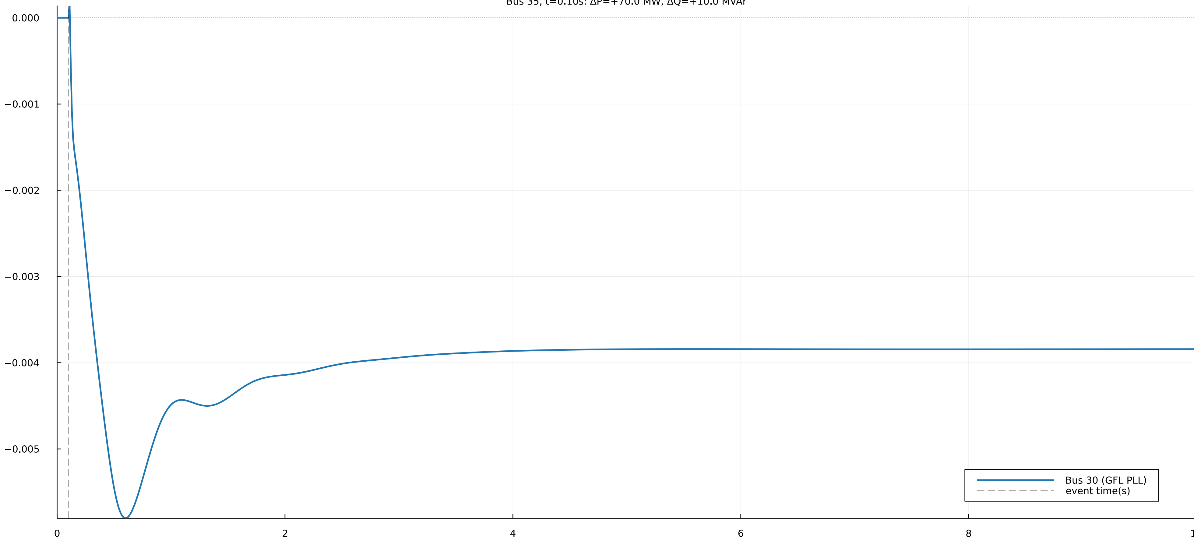
Frequency deviation at bus 30 Bus 35, t=0.10s: \Delta P=+70.0 MW, \Delta Q=+10.0 MVar
