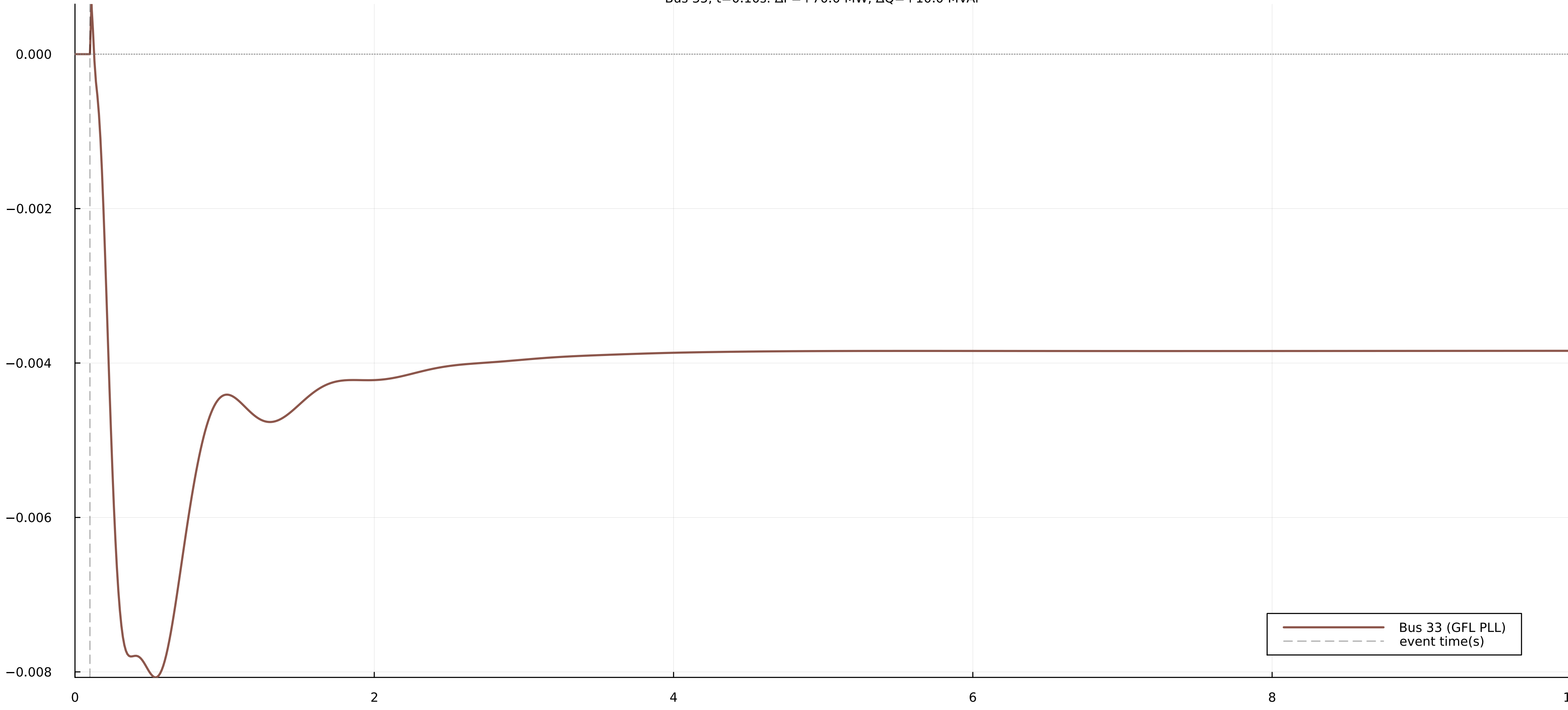
Frequency deviation at bus 33 Bus 35, t=0.10s: \Delta P=+70.0 MW, \Delta Q=+10.0 MVar
