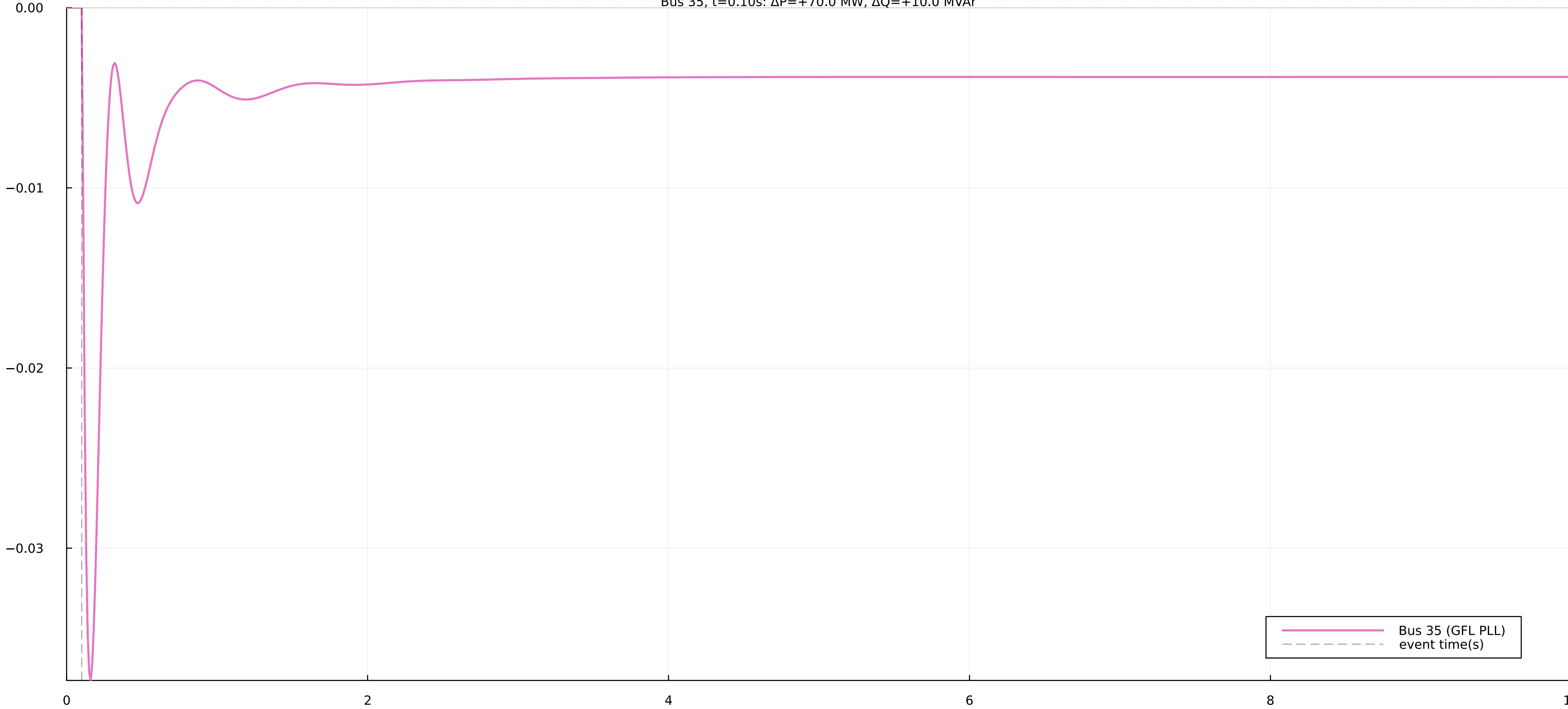
Frequency deviation at bus 35 Bus 35, t=0.10s: \Delta P=+70.0 MW, \Delta Q=+10.0 MVar
